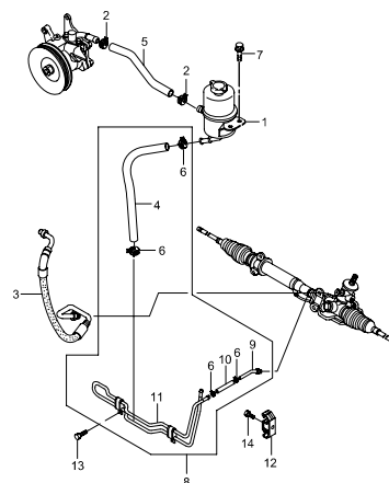
4640 POWER STEERING PIPE LINE(OLD)
