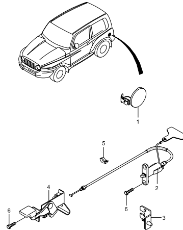
7090 FUEL FILLER DOOR LOCK
