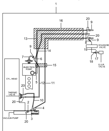
1620 VACUUM SYSTEM(OM600;M/T)
