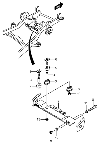
4310 FRONT AXLE MOUNTING
