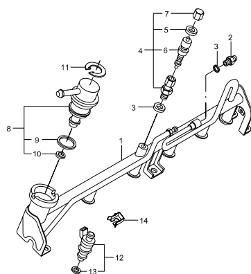
2242 FUEL SYSTEM(E32)
