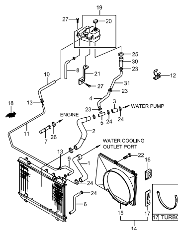
2130 RADIATOR HOSE & PIPE
