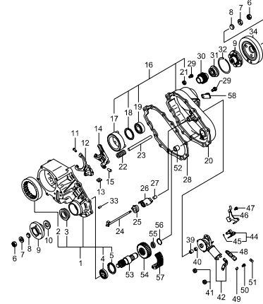
3212 TRANSFER CASE;PART TIME(2)
