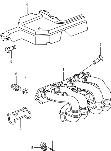
1712 INTAKE MANIFOLD(E20,E23)
