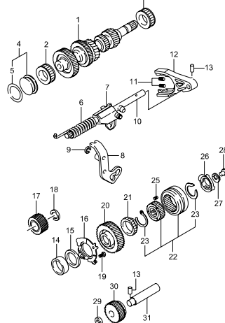
3152 COUNT SHAFT GEAR-T5(4WD)
