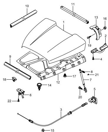
6110 HOOD PANEL
