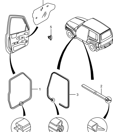
7121 FRONT WEATHER STRIP
