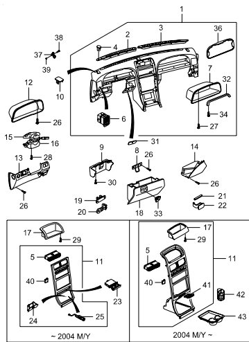
7610 INSTRUMENT PANEL
