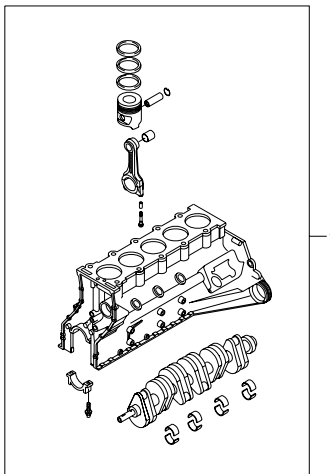
1120 SHORT BLOCK(DSL)
