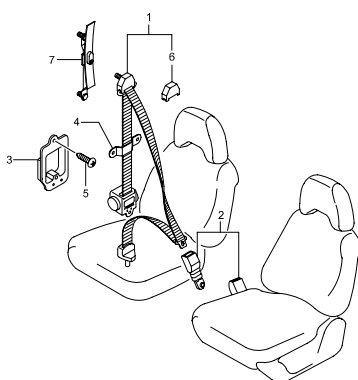
7430 FRONT SEAT BELT
