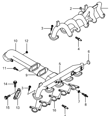
1711 INTAKE MANIFOLD(OM662,OM662LA)
