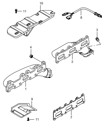
1723 EXHAUST MANIFOLD(E32)
