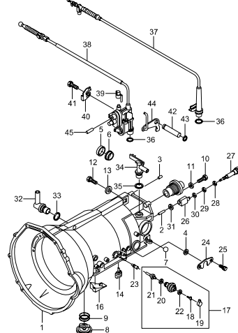
3612 TRANSMISSION HOUSING(W4A040)
