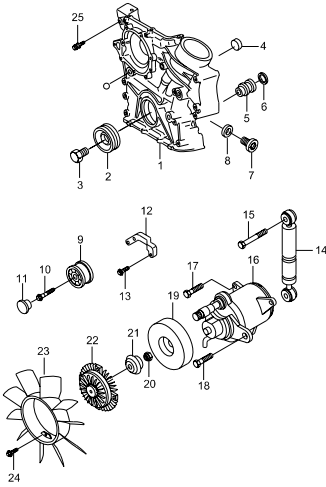
1331 TIMING CASE(E20,E23)
