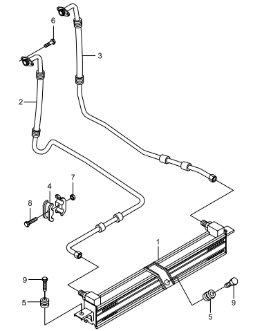
1550 ENGINE OIL COOLER
