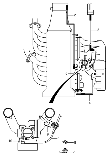
1624 VACUUM SYSTEM(E32)
