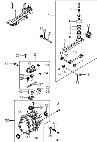
3176 SHIFTER & EXTENSION-TSM54(M/T,4WD)
