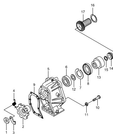
3642 TRANSMISSION HOUSING(BTR M74)
