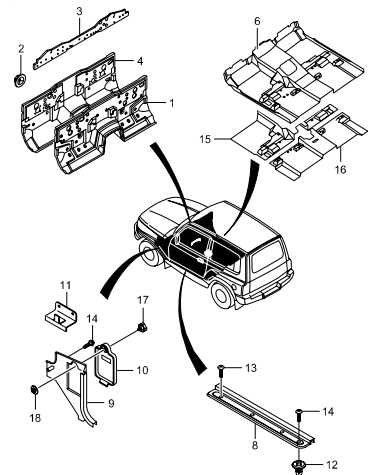
7720 FRONT FLOOR CARPET
