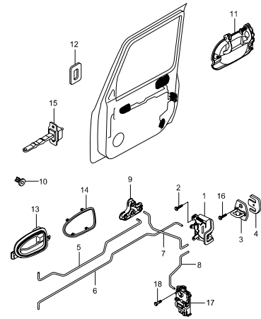
7110 FRONT DOOR OPENING SYSTEM
