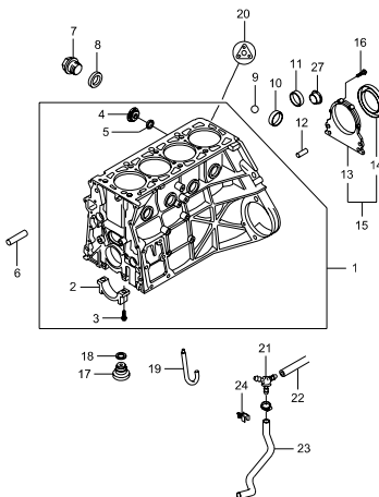
1123 CYLINDER BLOCK(E20,E23)
