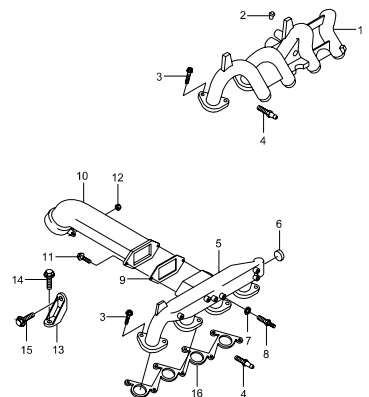
1710 INTAKE MANIFOLD(OM661,OM661LA)
