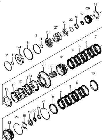
3645 CLUTCH(BTR M74)
