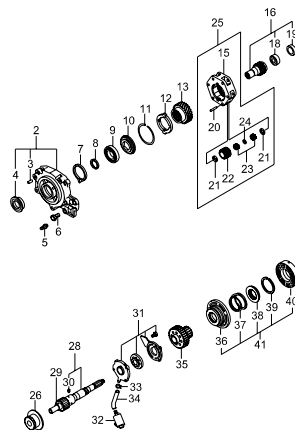
3211 TRANSFER CASE;PART TIME(1)
