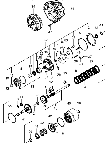
3641 CONVERTER HOUSING & OIL PUMP(BTR M74)
