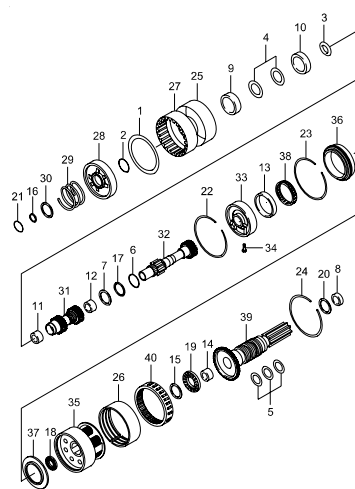
3646 OUTPUT SHAFT(BTR M74)
