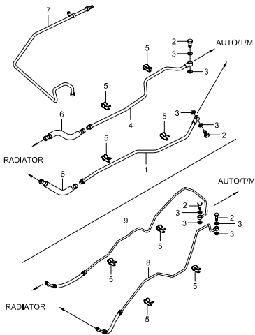
3750 AUTO COOLING SYSTEM
