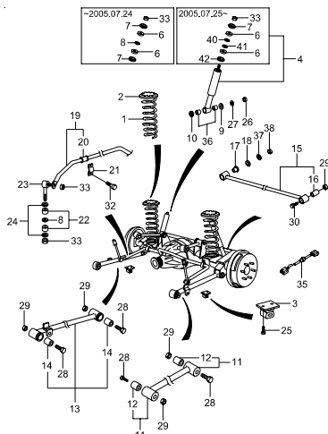
4511 REAR SHOCK ABSORBER
