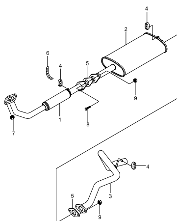
2410 EXHAUST SYSTEM(DSL)
