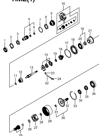
3221 TRANSFER CASE;FULL TIME(1)
