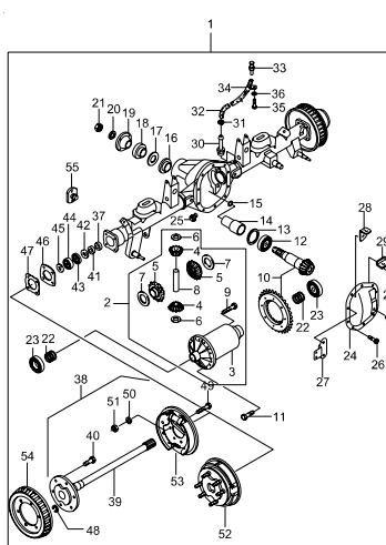
4211 REAR AXLE(TONGIL)
