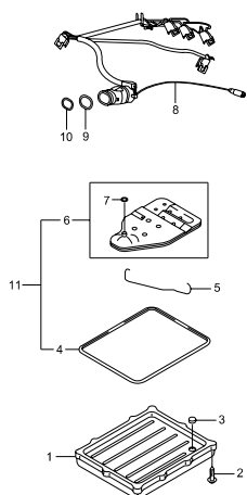
3644 OIL PAN(BTR M74)
