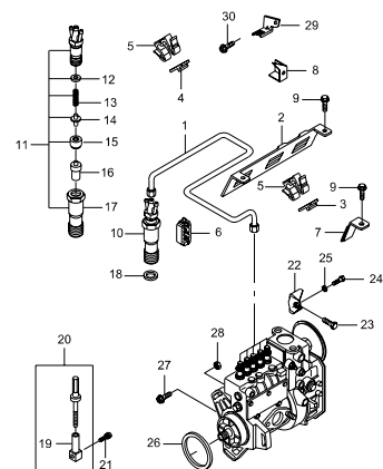
1830 INJECTION PIPE BRACKET & NOZZLE(OM600)
