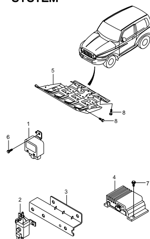
3420 ELECTRIC CONTROL SYSTEM
