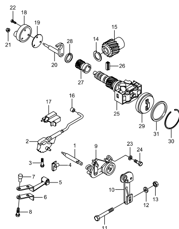
3616 STARTER I/LOCK S/W & GOVERNOR(W4A040)
