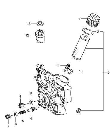
1541 OIL FILTER(E20,E23)
