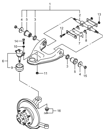
4410 FRONT SUSPENSION
