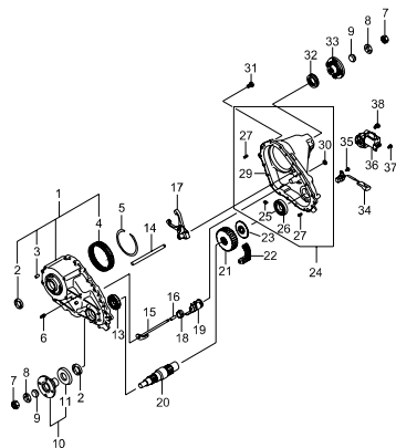
3222 TRANSFER CASE;FULL TIME(2)
