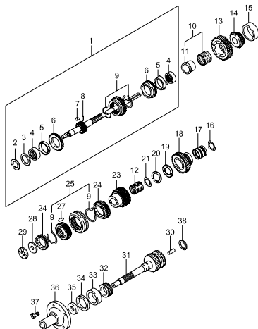
3151 OUTPUT & INPUT SHAFT-T5(4WD)
