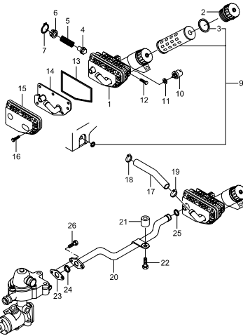
1542 OIL FILTER(E32)
