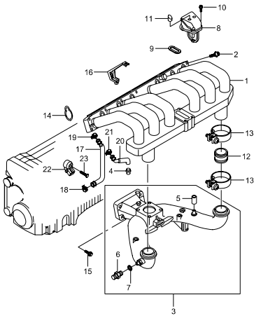
1713 INTAKE MANIFOLD(E32)
