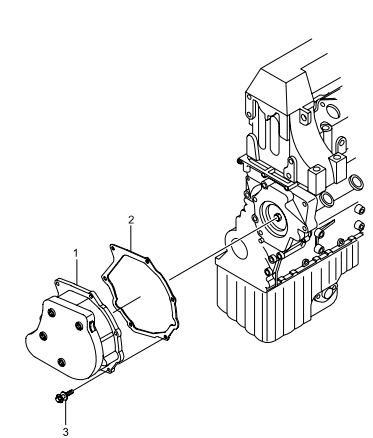
1610 VACUUM PUMP(DSL)
