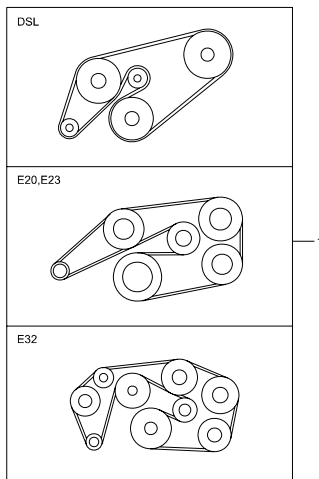
1350 BELT SYSTEM
