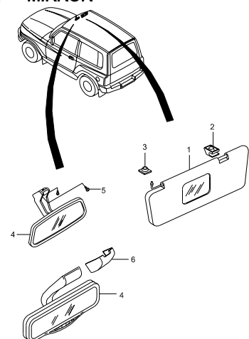
7770 SUNSHADE & INSIDE MIRROR
