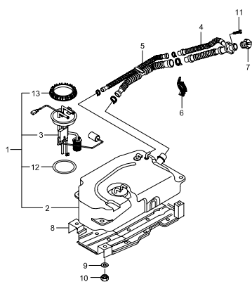
2210 FUEL TANK(DSL)
