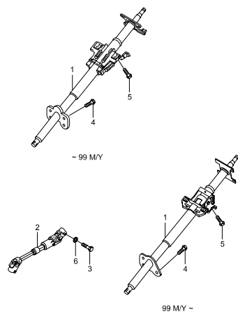
4613 STEERING COLUMN
