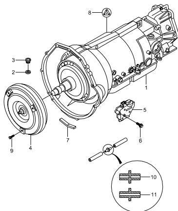
3610 AUTOMATIC TRANSMISSION(W4A040)
