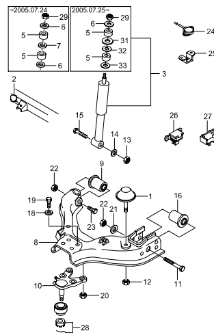
4411 FRONT SHOCK ABSORBER
