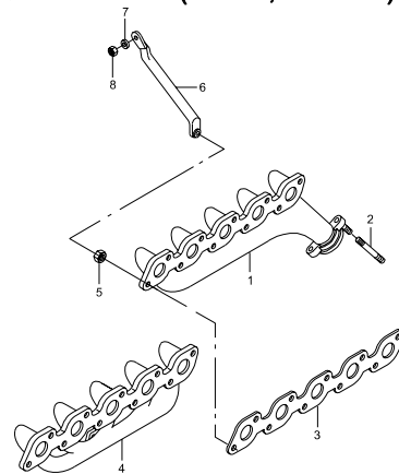
1721 EXHAUST MANIFOLD(OM662,OM662LA)
