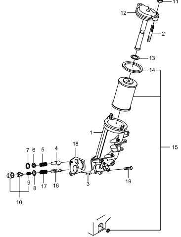
1540 OIL FILTER & COOLER(OM600)
