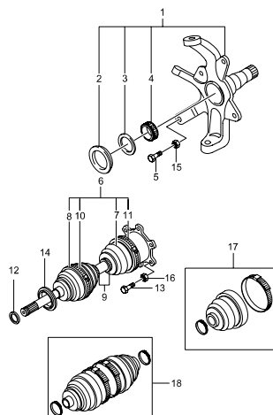
4110 AXLE SHAFT
