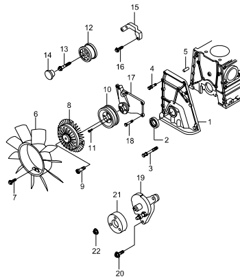
1332 TIMING CASE(E32)
