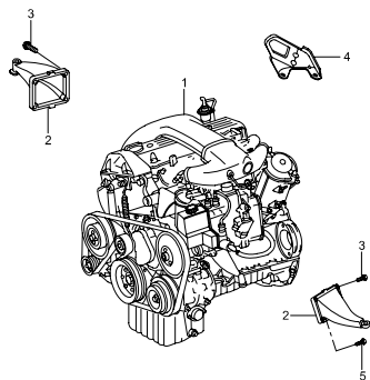
1110 ENGINE UNIT(OM661,OM661LA)
