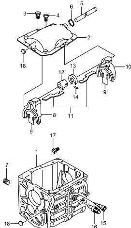
3153 TRANSMISSION CASE-T5(4WD)
