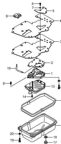
3614 OIL PAN(W4A040)
