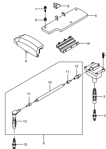
1440 IGNITION COIL(E20,E23)
