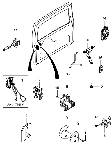
7310 TAIL GATE LOCK
