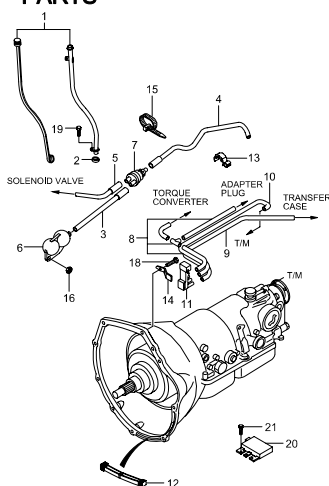
3670 POWER TRAIN AUXILIARY PARTS
