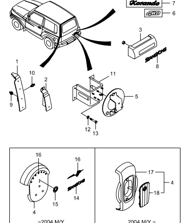
7321 REAR END TRIM
