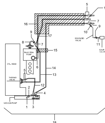
1622 VACUUM SYSTEM(OM600)
