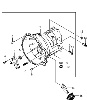
3171 CLUTCH HOUSING-TSM54(M/T,4WD)
