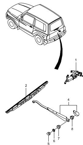
7830 BACK WINDOW WIPER
