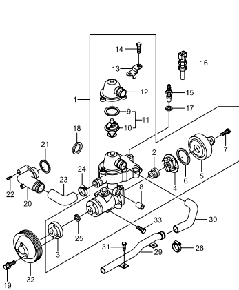
1522 COOLING SYSTEM(E32)
