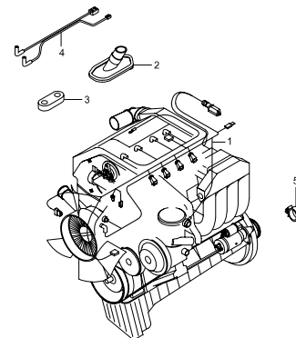
1411 ENGINE WIRING(GSL)
