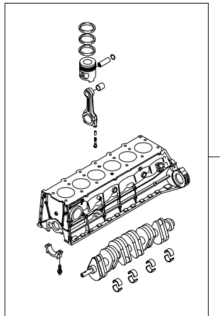
1121 SHORT BLOCK(GSL)
