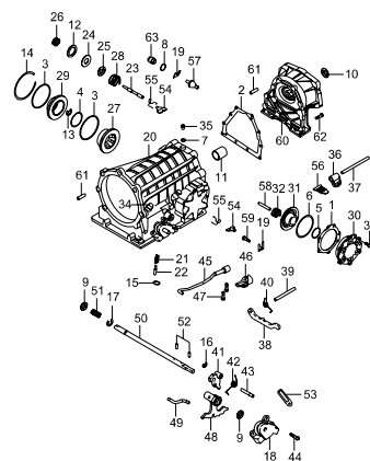
3642 TRANSMISSION HOUSING(BTR M74)
