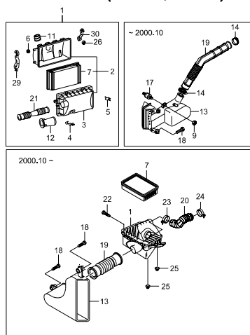
2310 AIR CLEANER(OM661,OM662)
