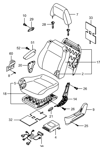
7420 FRONT SEAT PARTS
