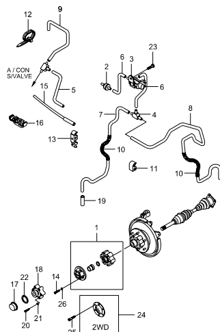
4116 LOCKING HUB
