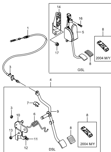
2010 ACCELERATOR CONTROL
