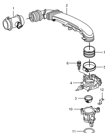
2320 AIR INTAKE SYSTEM(E20,E23)
