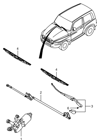
7810 WINDSHIELD WIPER
