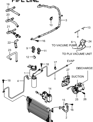
6820 AIR CONDITIONER HOSE & PIPE LINE
