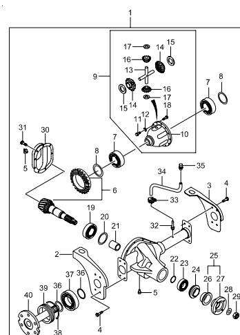
4121 FRONT AXLE(TONGIL)
