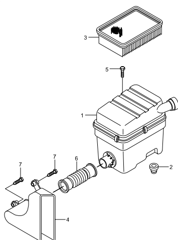
2312 AIR CLEANER(GSL)
