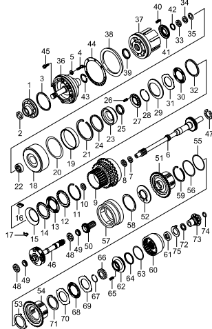
3611 OIL PUMP & INTERIOR PARTS(W4A040)
