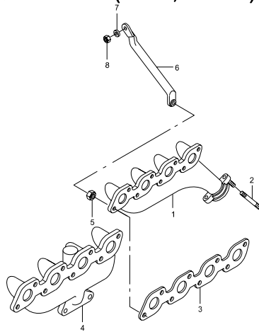
1720 EXHAUST MANIFOLD(OM661,OM661LA)
