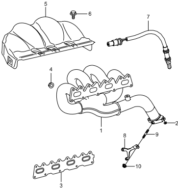
1722 EXHAUST MANIFOLD(E20,E23)
