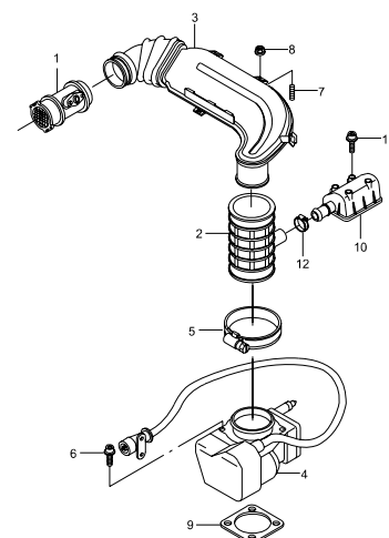
2321 AIR INTAKE SYSTEM(E32)
