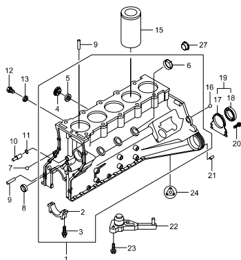
1122 CYLINDER BLOCK(OM600)
