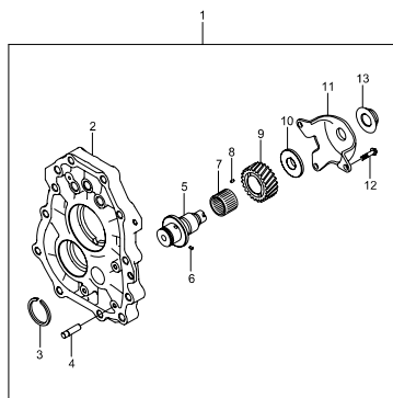
3174 ADAPTOR ASSY-TSM54(M/T,4WD)
