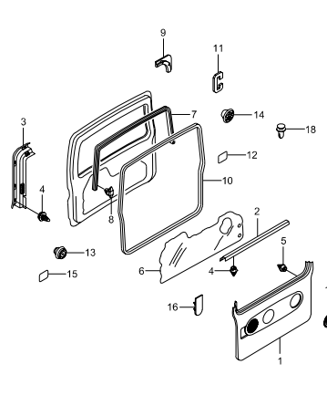
7320 TAIL GATE TRIM
