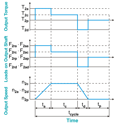
Motion Profile
