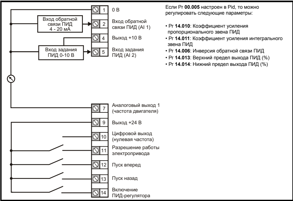
Рис. 4-17 Pr 00.005 = Pid (50 Гц)
