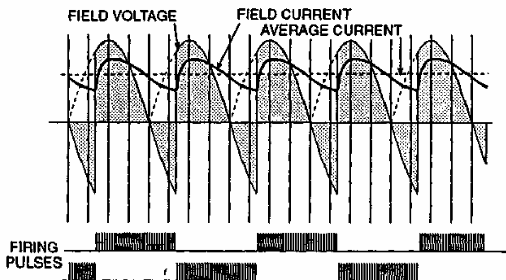
2 Full wave rectified voltage and current.
