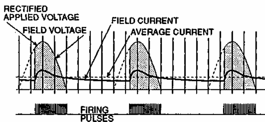
1 Half wave rectified voltage and current.
