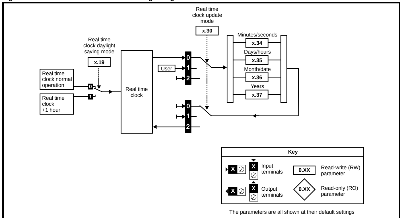
Figure 13-32 SM-I/O Timer real time clock logic diagram
