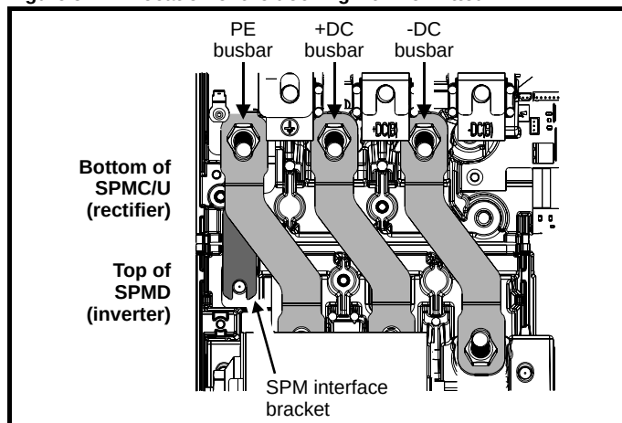
Figure 5-21 Location of the docking kit when fitted
