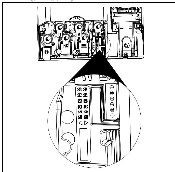
Figure 6-9 Heatsink fan supply connections (SPMA & SPMD)
