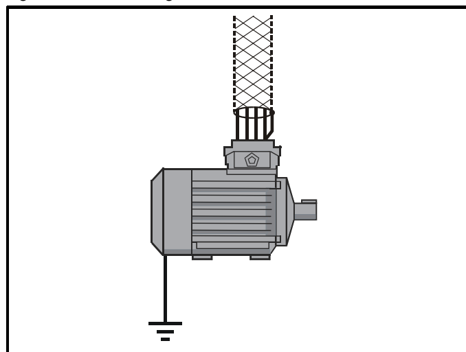
Figure 6-23 Grounding the motor cable shield
