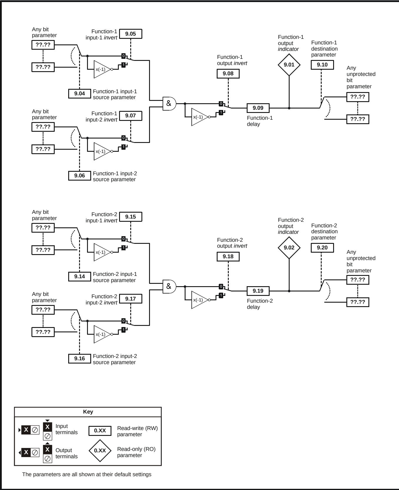
Figure 13-13 Menu 9 logic diagram
