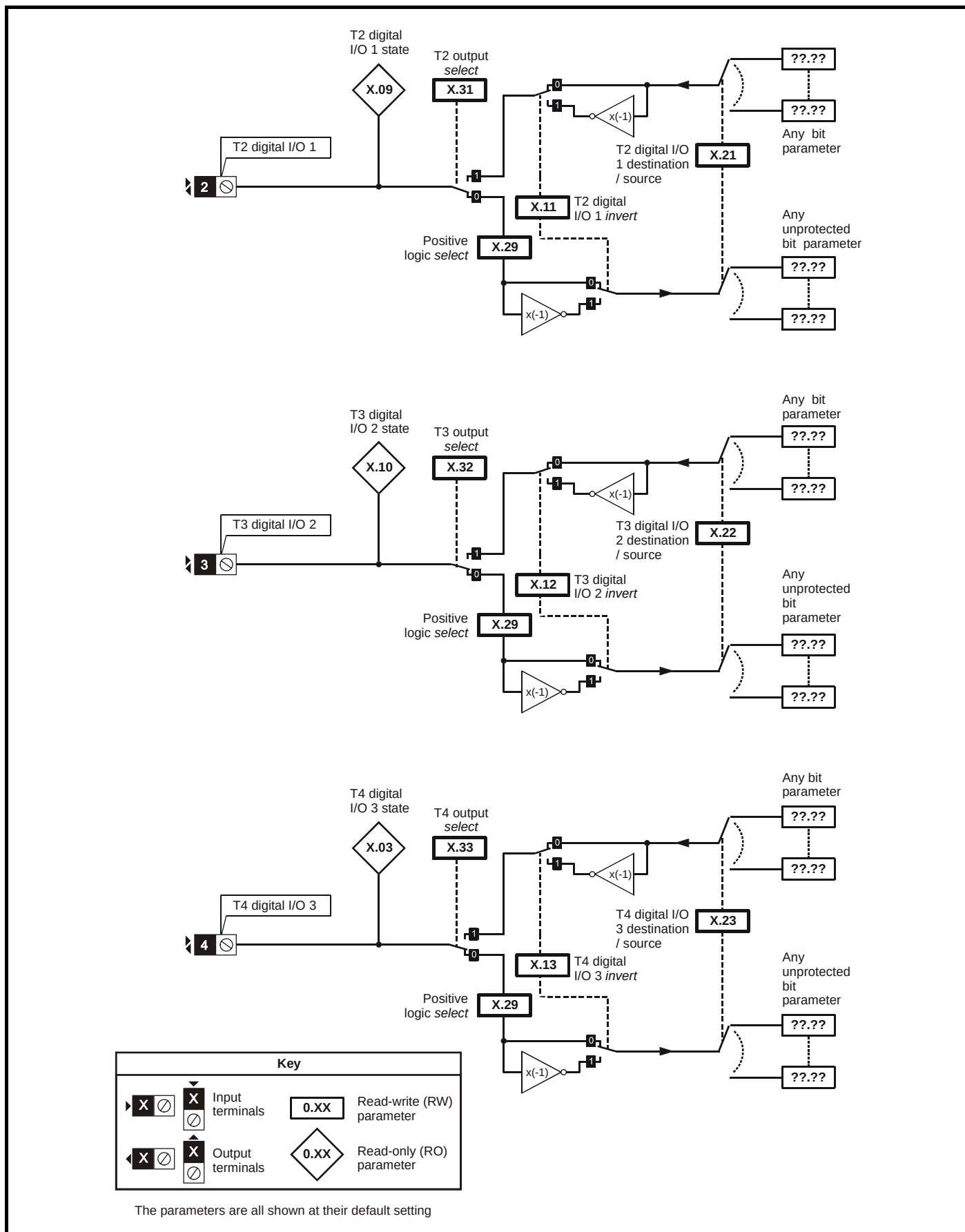
Figure 13-28 SM-I/O Plus digital logic diagram 1
