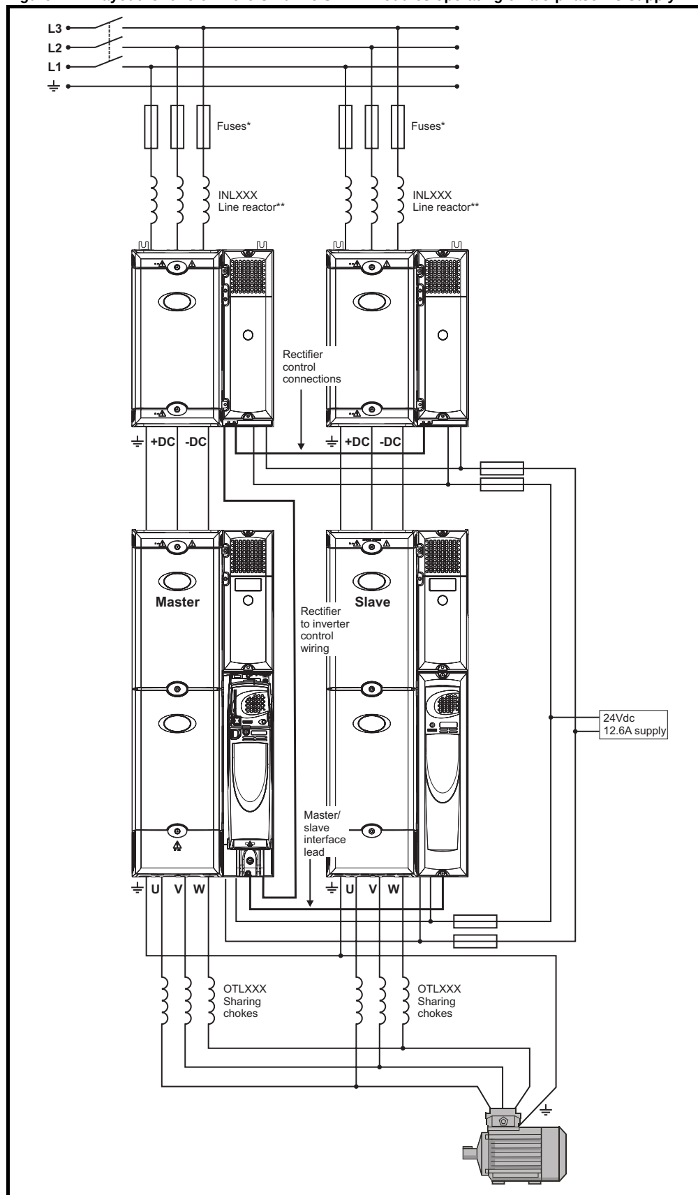
Figure 4-4 Layout for two or more Unidrive SPMD modules operating on a 3-phase AC supply
