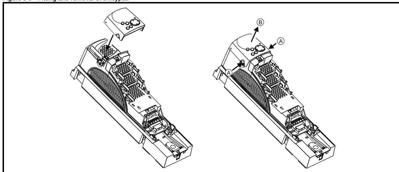
Figure 5-6 Fitting and removal of a keypad
