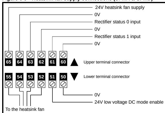
Figure 6-9 Heatsink fan supply connections (SPMA & SPMD)
