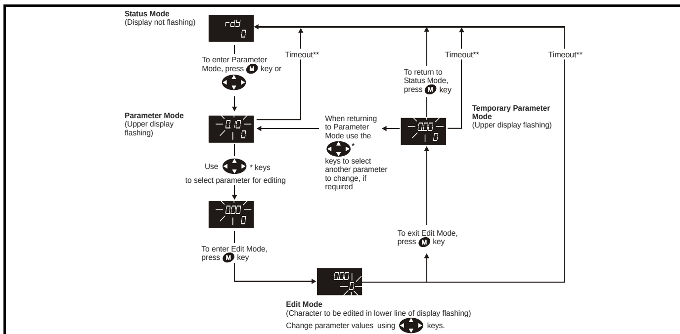
Figure 7-3 Display modes
