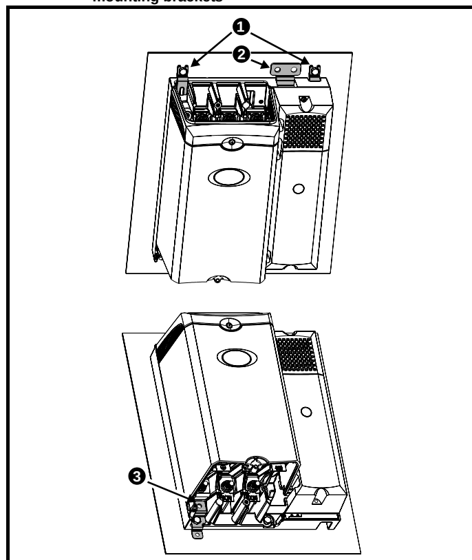
Figure 5-19 Fitting of the Unidrive SPMC/U through panel mounting brackets
