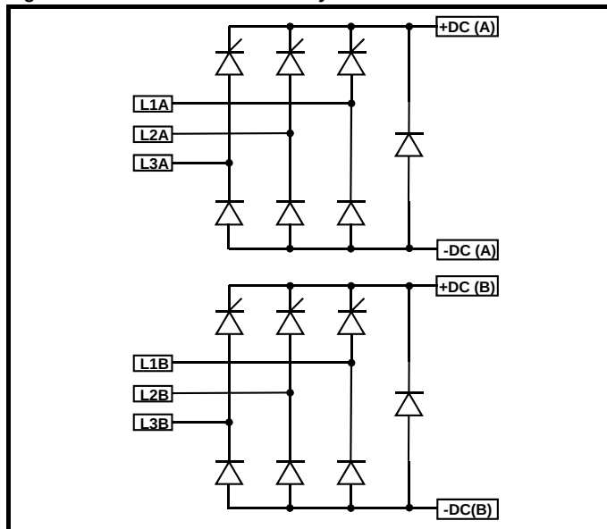
Figure 2-2 Dual half controlled thyristor
