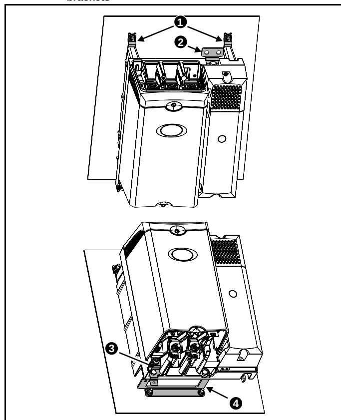
Figure 5-18 Fitting of the Unidrive SPMC/U surface mounting brackets
