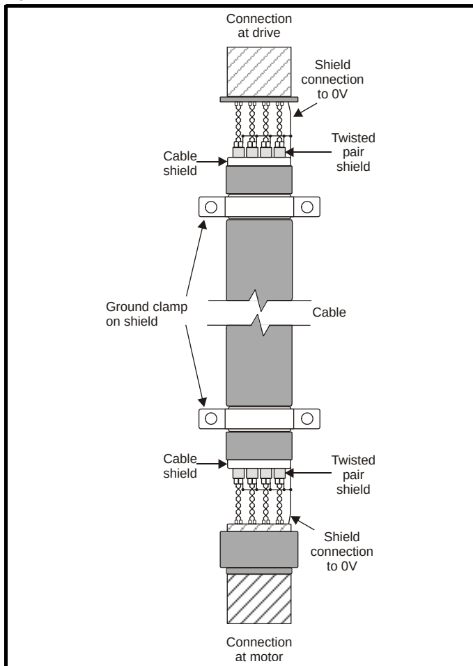
Figure 6-19 Feedback cable connections
