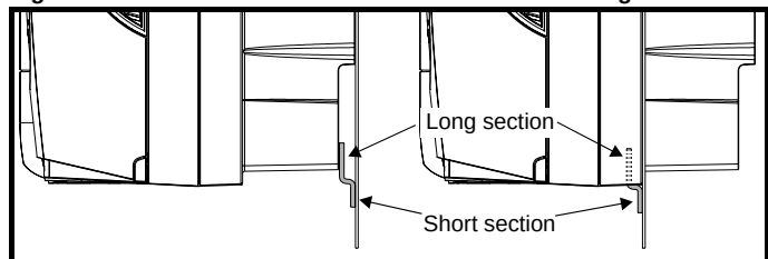
Figure 5-16 Orientation of the Unidrive SPM mounting bracket
