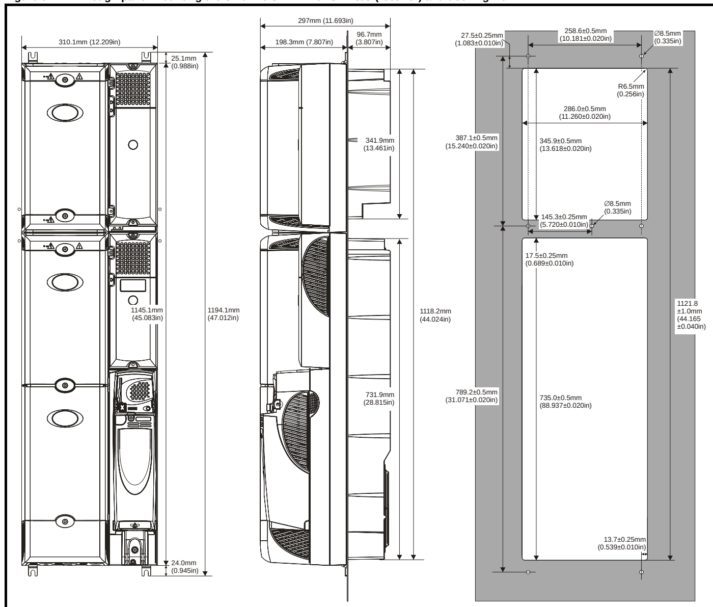
Figure 5-14 Through-panel mounting the Unidrive SPMD with SPMC/U (rectifier) and docking kit
