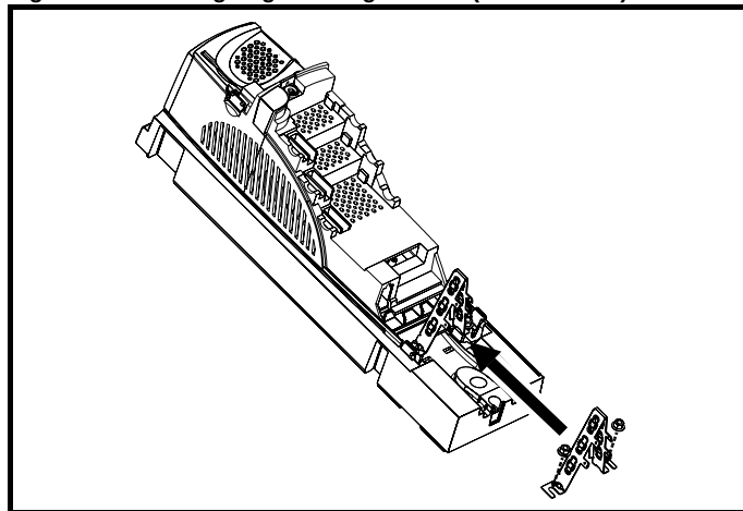
Figure 6-14 Fitting of grounding bracket (master/slave)
