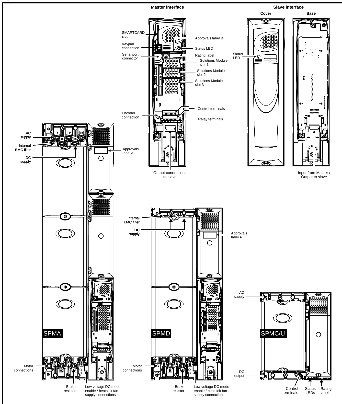
Figure 3-1 Features of the Unidrive SPM Modules
