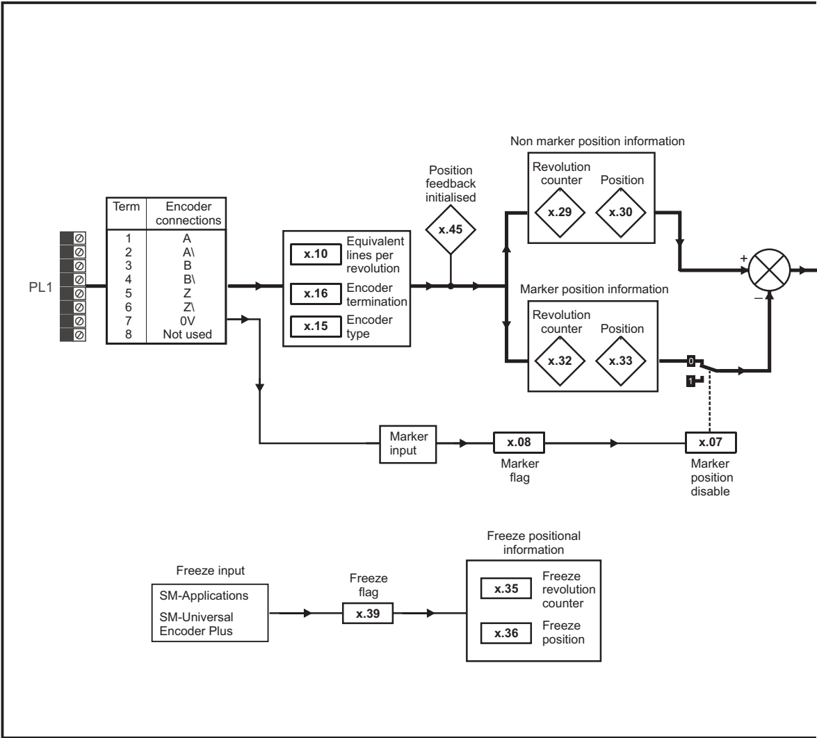
Figure 13-26 SM-Encoder Plus logic diagram
