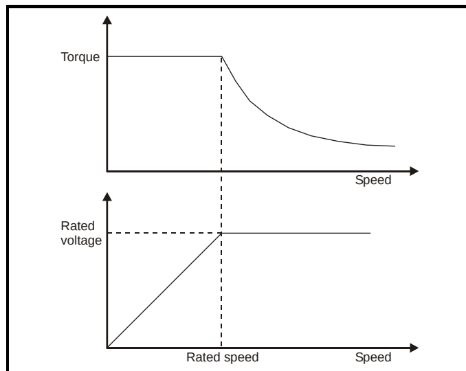
Figure 10-3 Torque and rated voltage against speed
