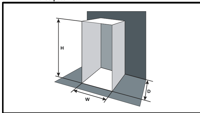
Figure 5-24 Enclosure having front, sides and top panels free to dissipate heat
