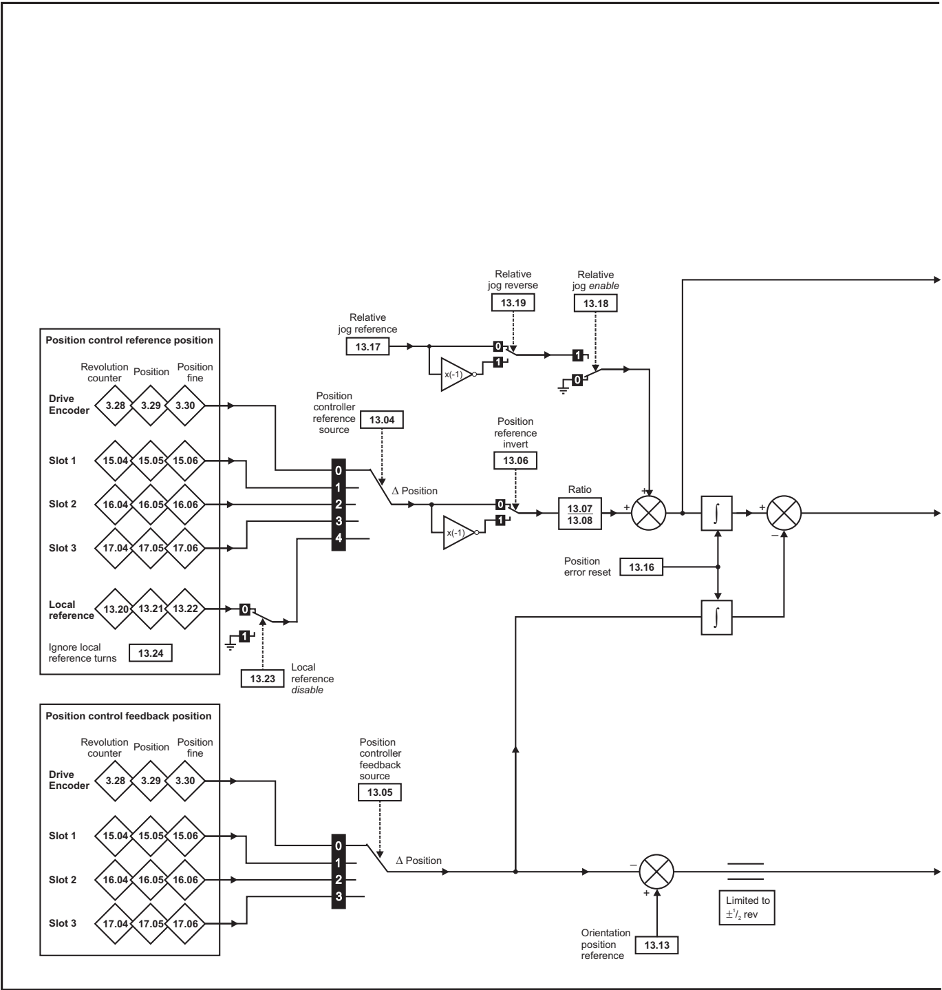
Figure 13-21 Menu 13 Closed-loop logic diagram
