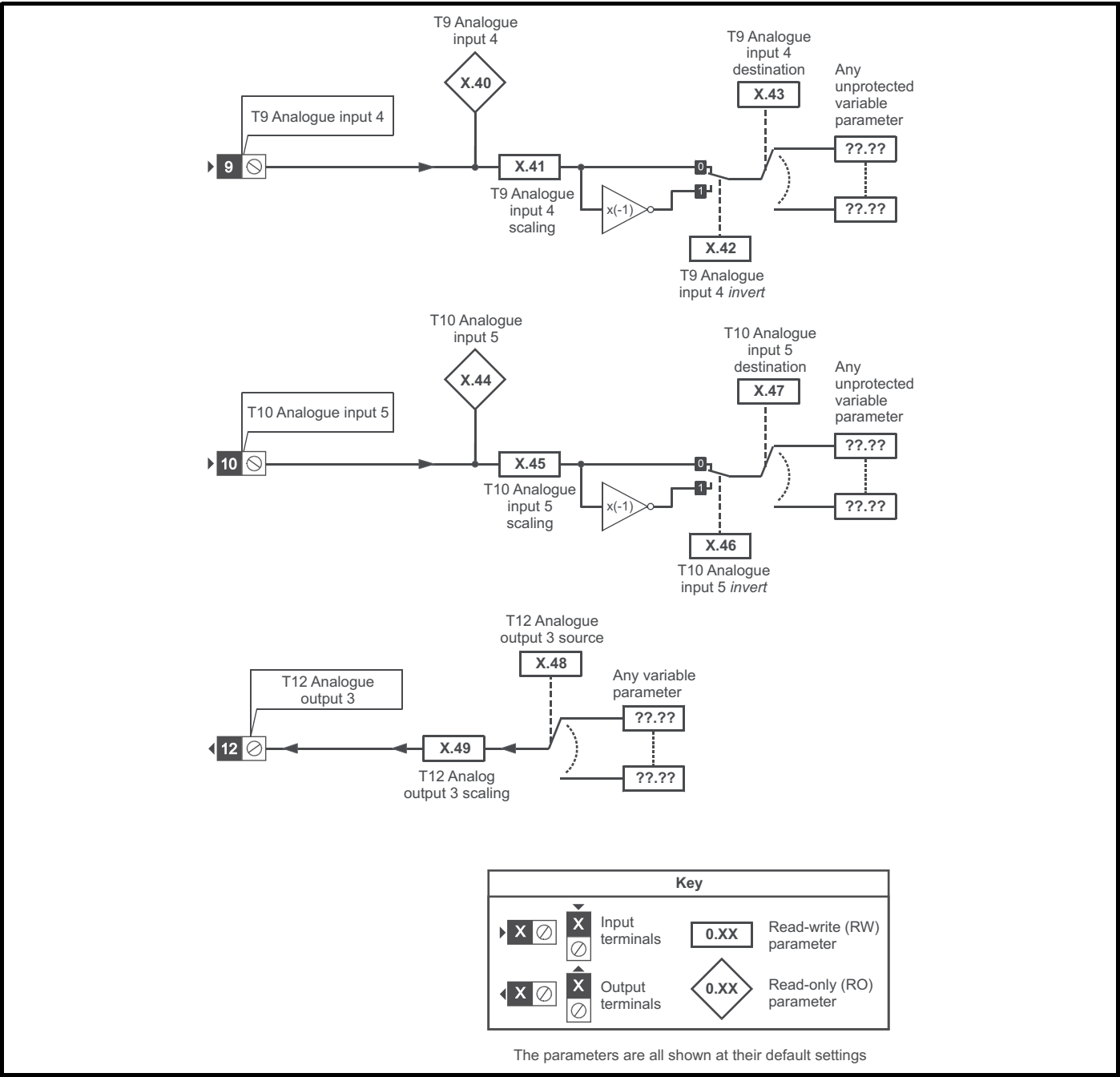
13.15.3 Automation module category Figure 13-27 SM-I/O Plus analogue logic diagram
