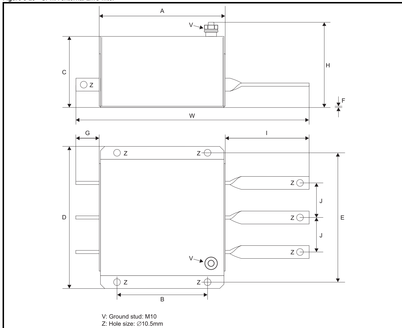
Figure 5-29 SPMA external EMC filter
