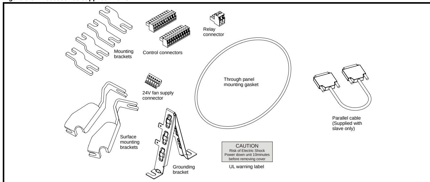
Figure 3-6 Accessories supplied with SPMD
