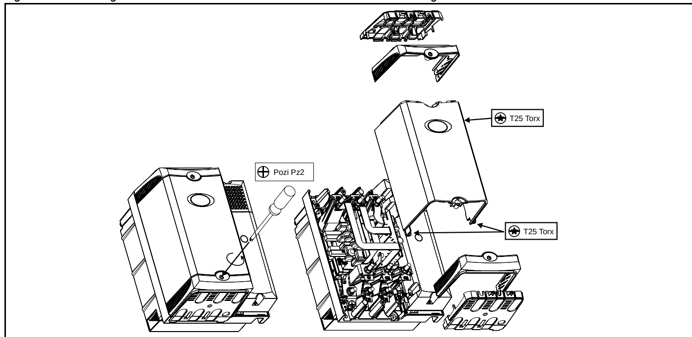
Figure 5-3 Removing the Unidrive SPMC/U dual rectifier terminal covers and housing
