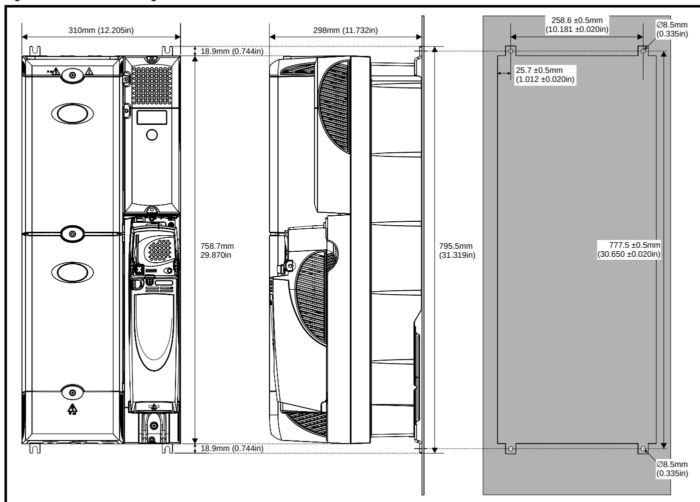
Figure 5-9 Surface mounting the Unidrive SPMC/U (rectifier)
