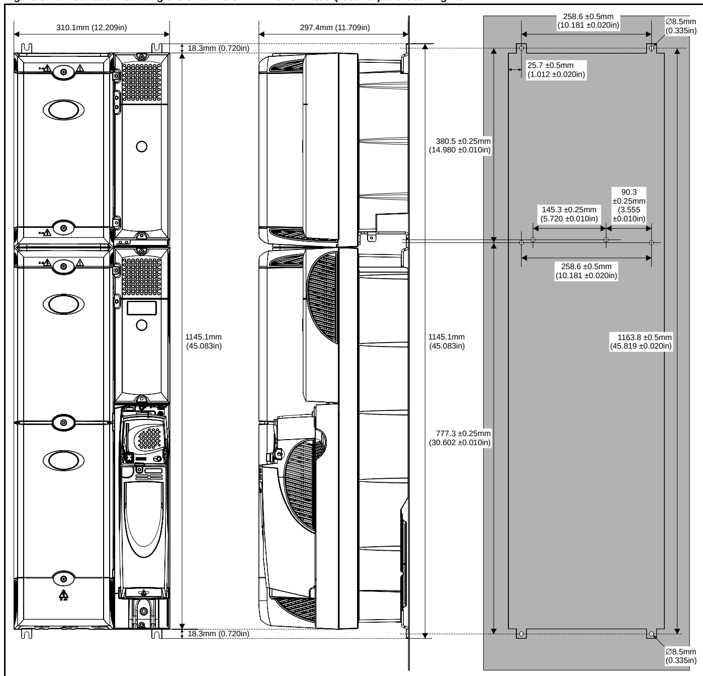
Figure 5-10 Surface mounting the Unidrive SPMD with SPMC/U (rectifier) and docking kit
