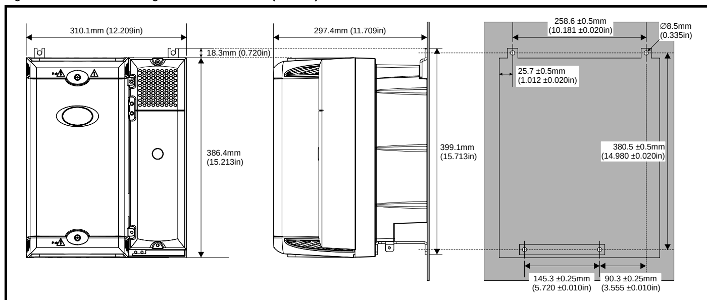
Figure 5-9 Surface mounting the Unidrive SPMC/U (rectifier)
