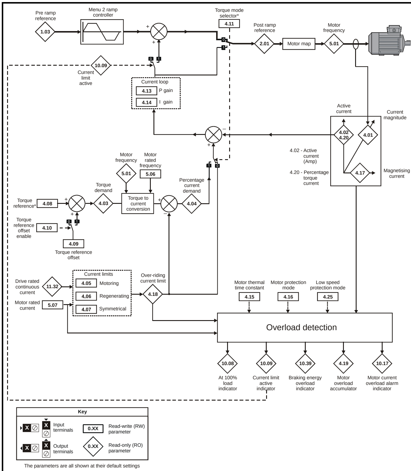
Figure 13-5 Menu 4 Open loop logic diagram
