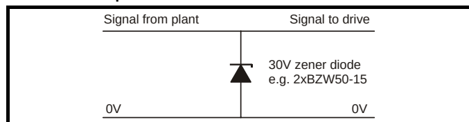
Figure 6-30 Surge suppression for analogue and bipolar inputs and outputs
