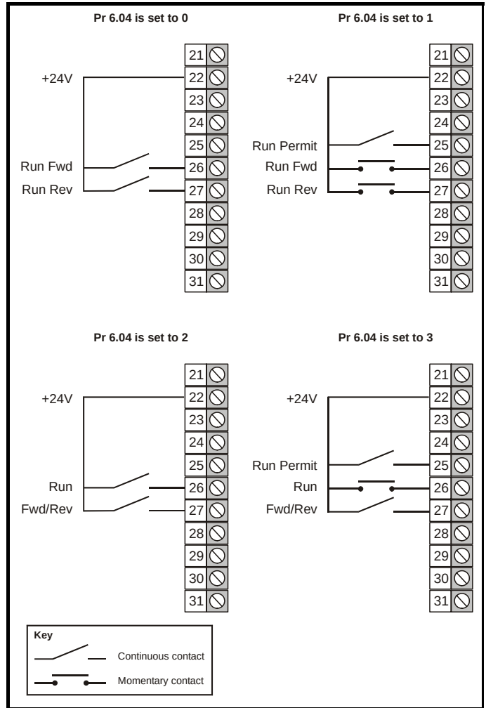
Figure 13-41 Digital input connections when Pr 6.04 is set to 0 to 3
