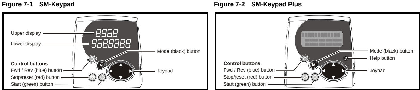
Figure 7-1 SM-Keypad
