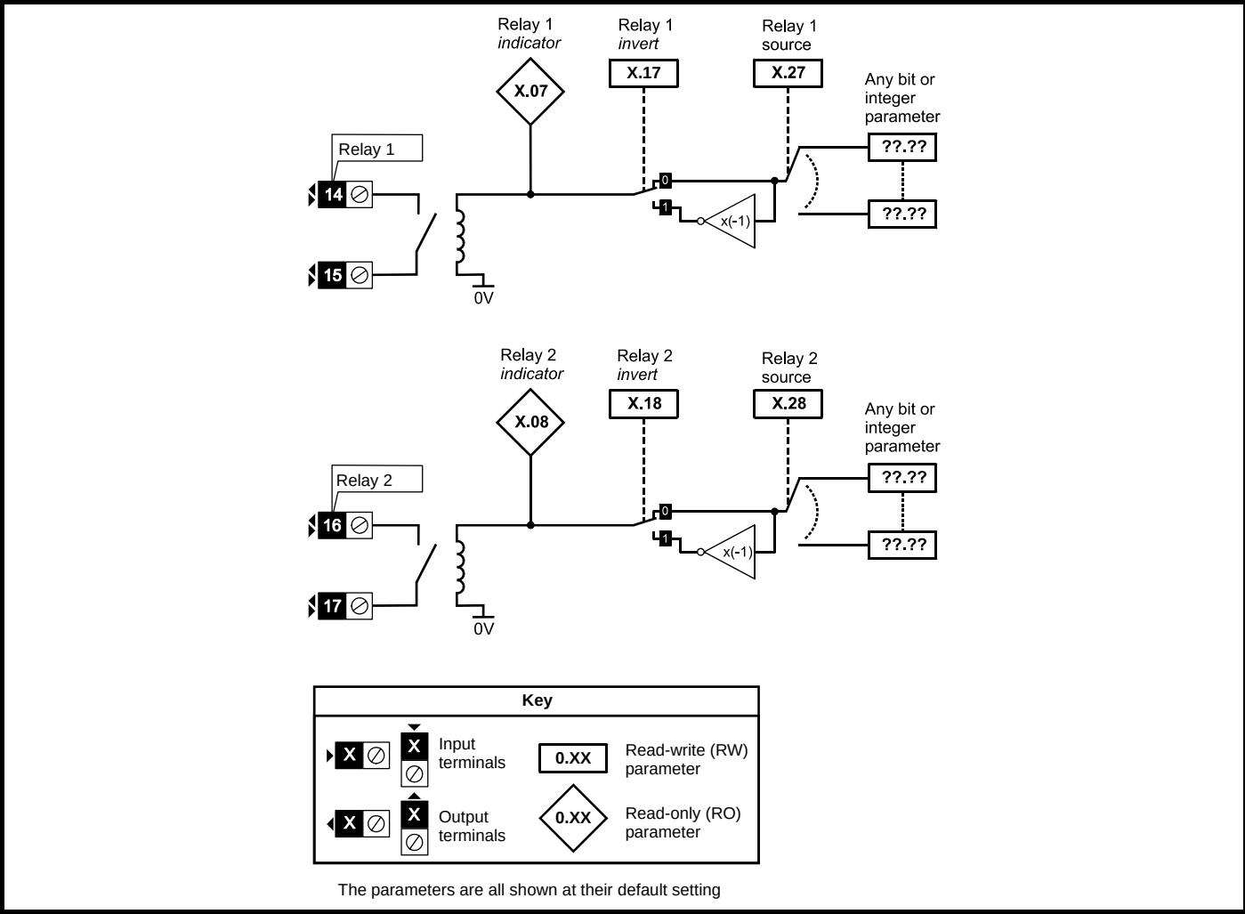
Figure 13-35 SM-PELV relay logic diagram
