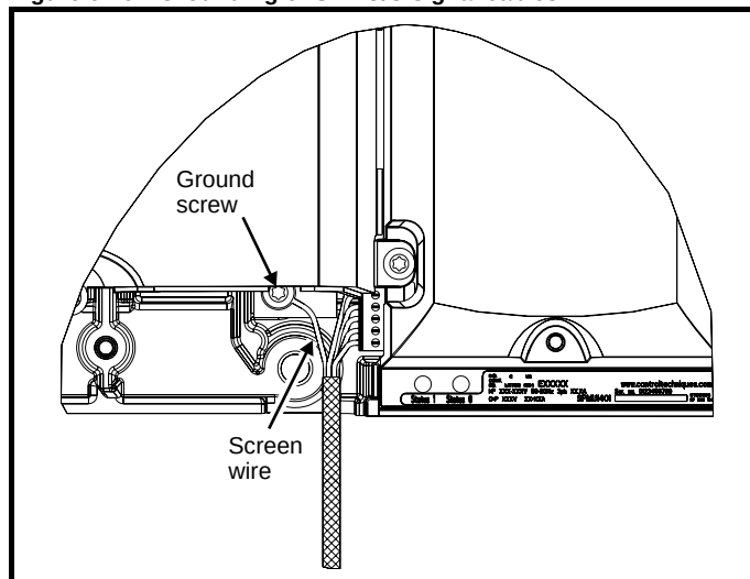
Figure 6-26 Grounding of SPMC/U signal cables
