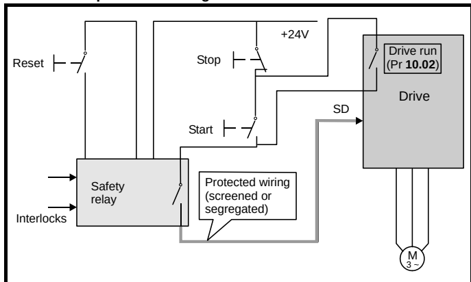
Figure 6-42 Category 3 interlock using Secure Disable with protected wiring
