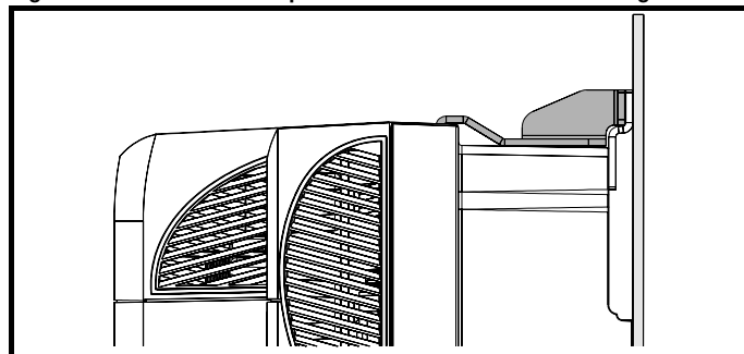
Figure 5-17 Location of top Unidrive SPMA surface mounting brackets
