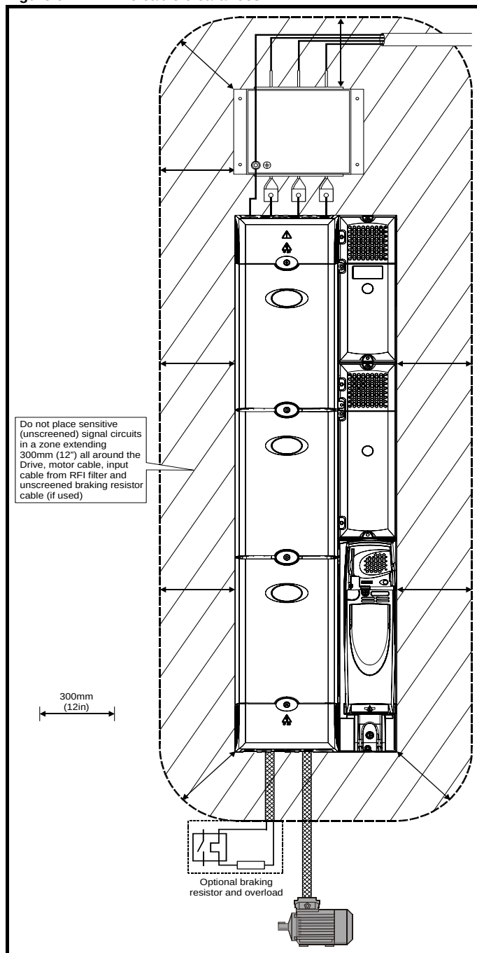
Figure 6-17 Drive cable clearances
