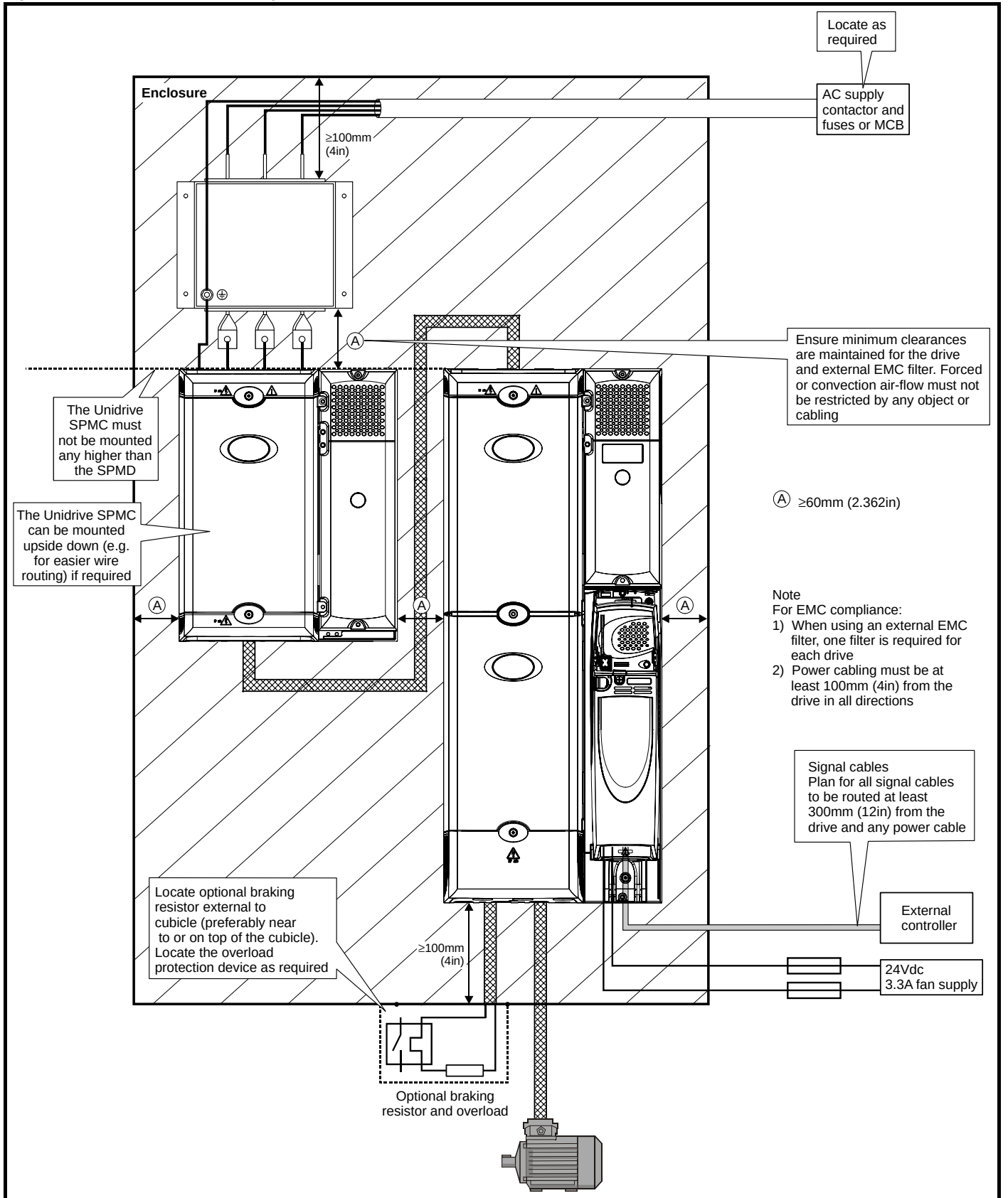
Figure 5-23 Alternative enclosure layout: Undocked Undrive SPMD and SPMC
