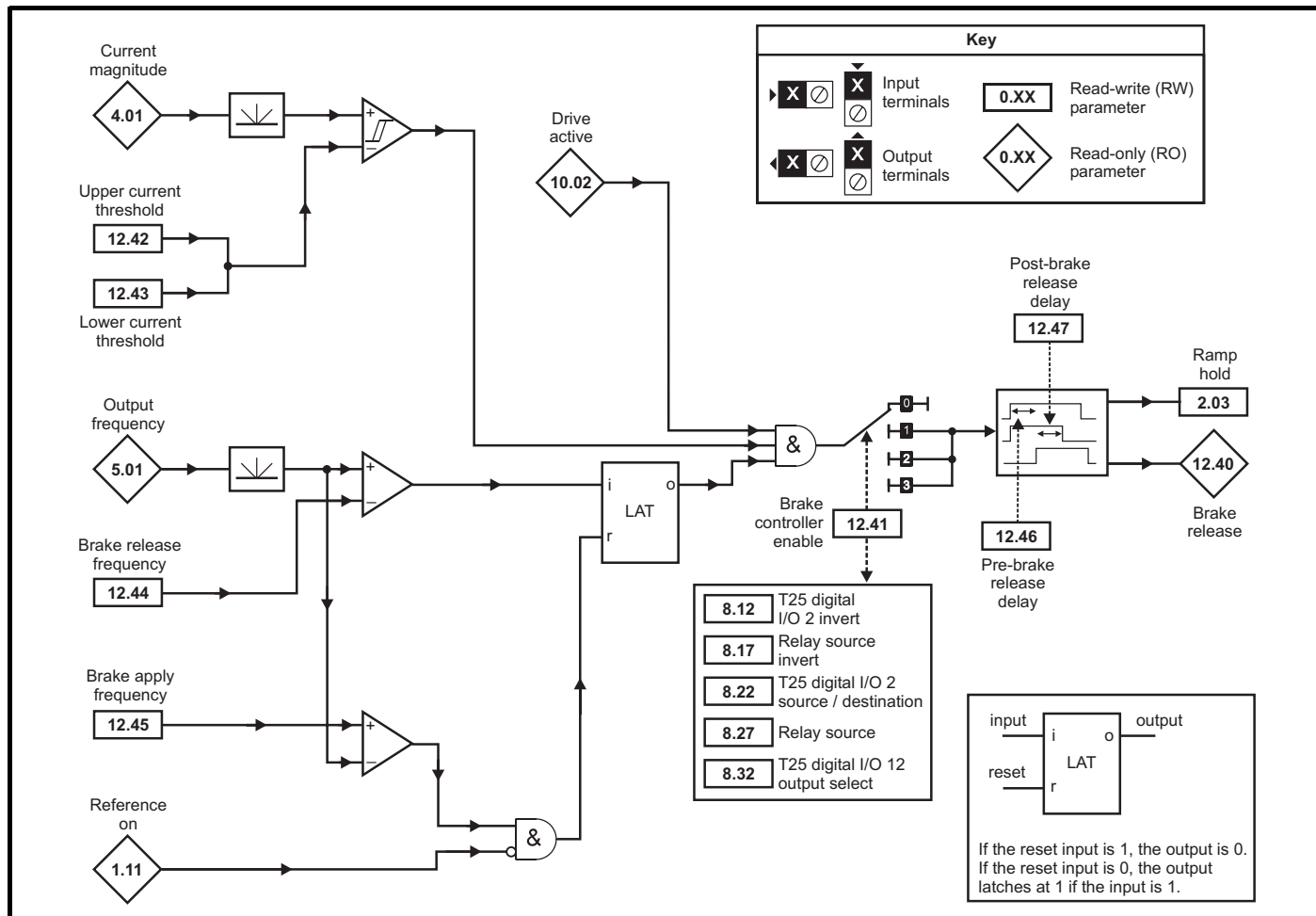
Figure 13-17 Open-loop brake sequence
