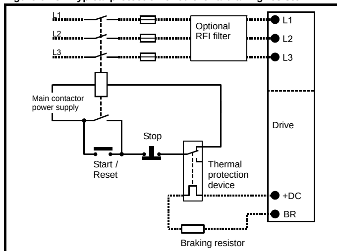
Figure 6-13 Typical protection circuit for a braking resistor
