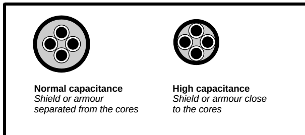
Figure 6-10 Cable construction influencing the capacitance
