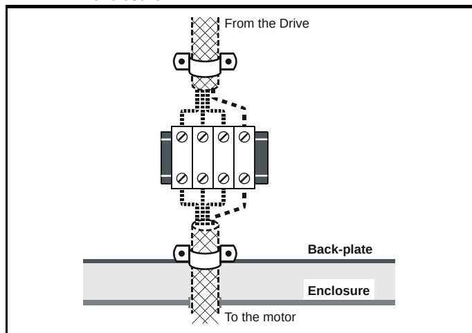
Figure 6-27 Connecting the motor cable to a terminal block in the enclosure
