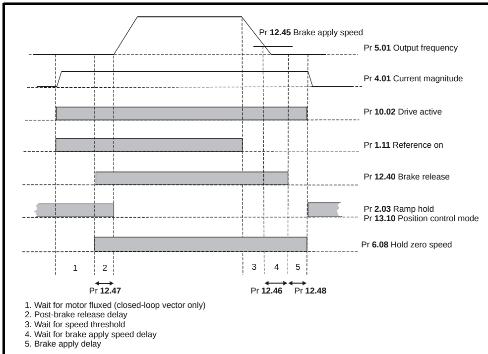
Figure 13-19 Closed-loop brake sequence
