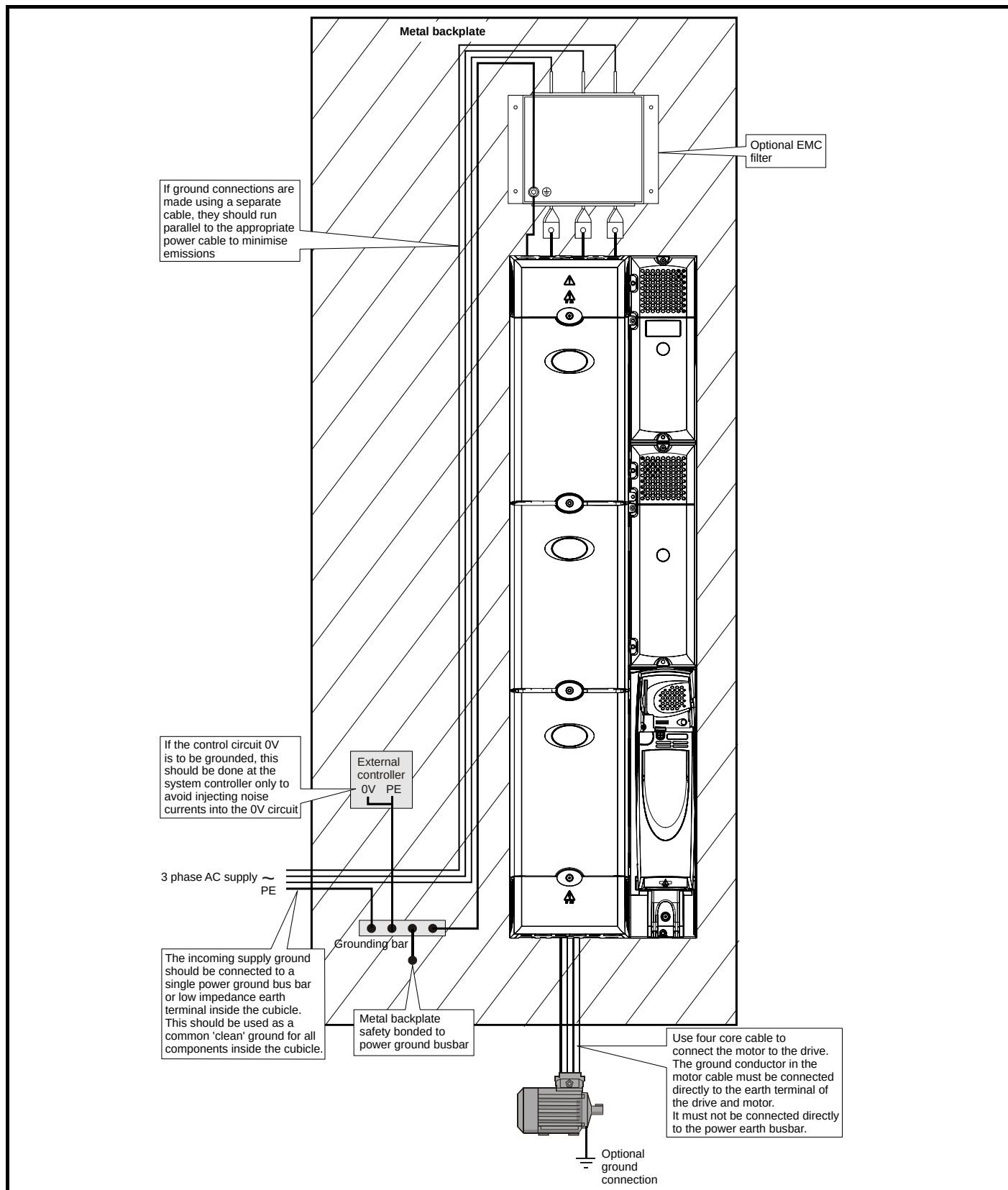
Figure 6-16 General EMC enclosure layout showing ground connections
