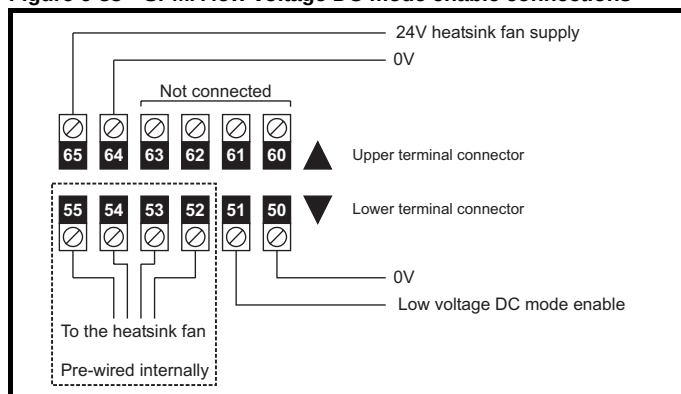
Figure 6-39 SPMD low voltage DC mode enable connections
