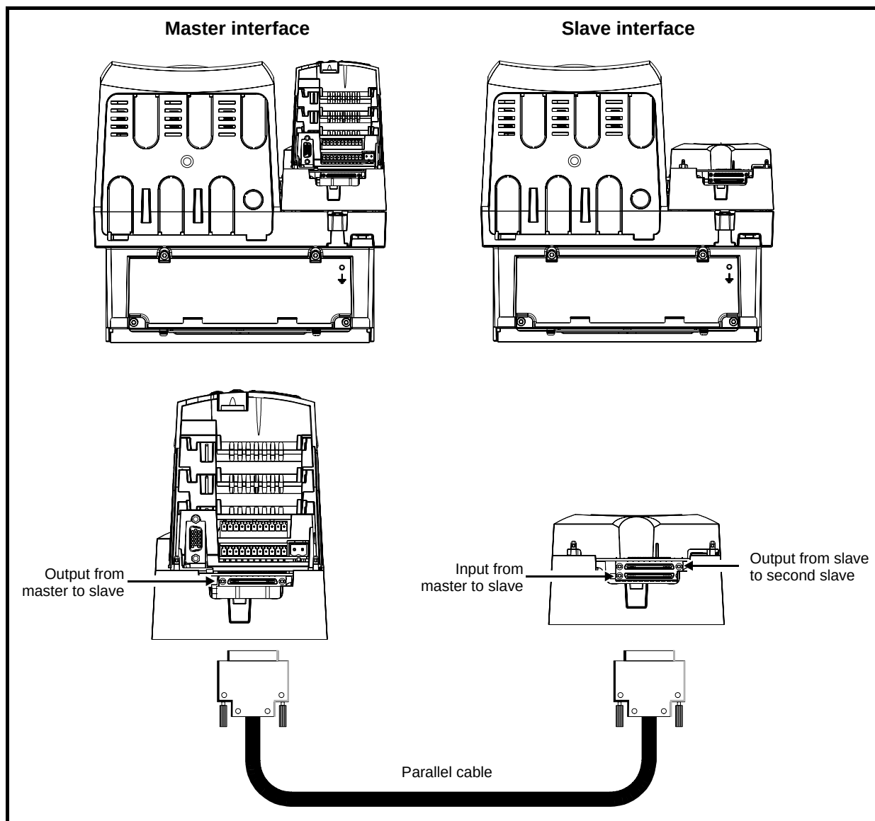
Figure 4-5 Parallel control connections
