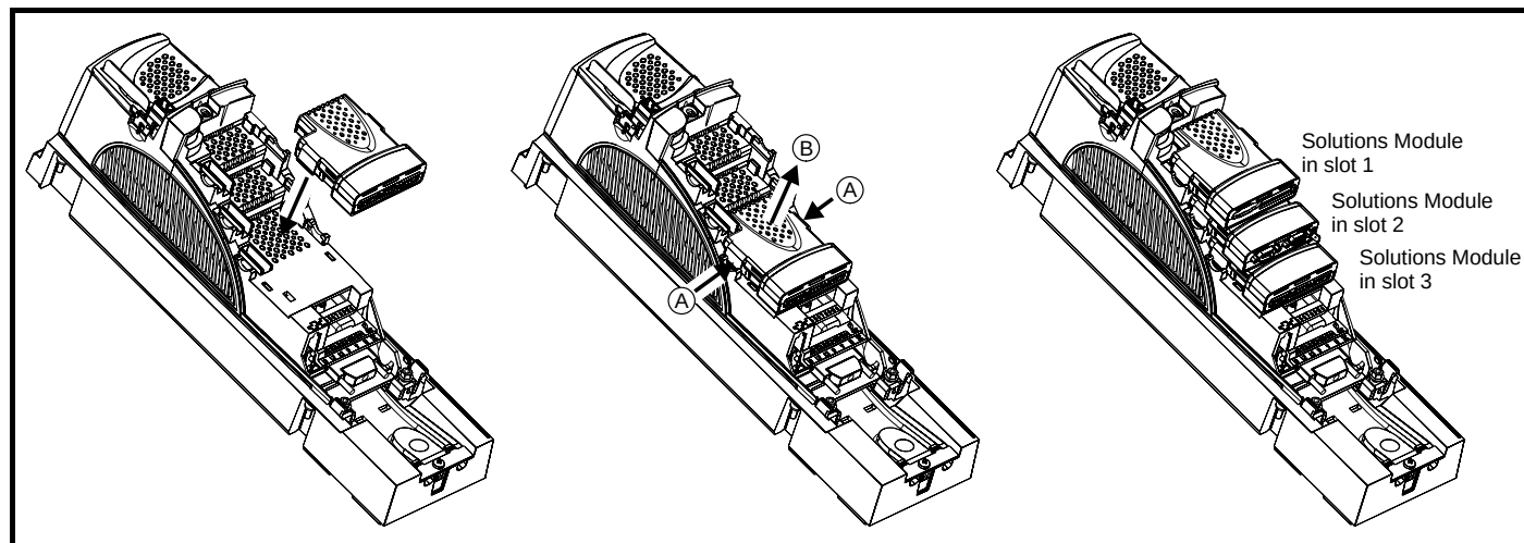
Figure 5-5 Fitting and removal of a Solutions Module
