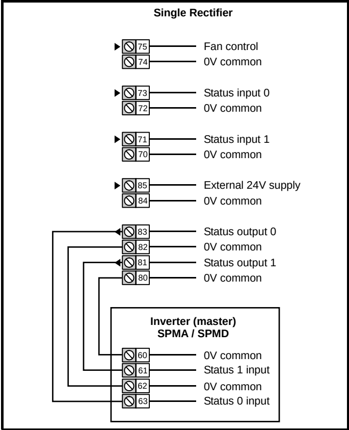
Figure 6-32 Single rectifier control terminals and descriptions
