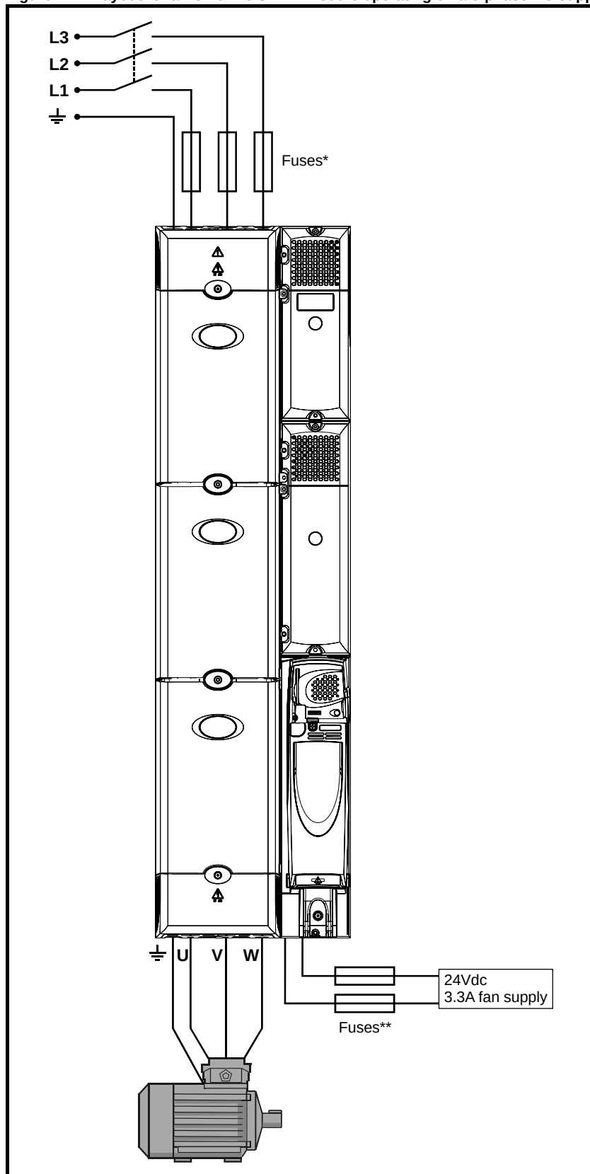
Figure 4-1 Layout for an Unidrive SPMA module operating on a 3-phase AC supply
