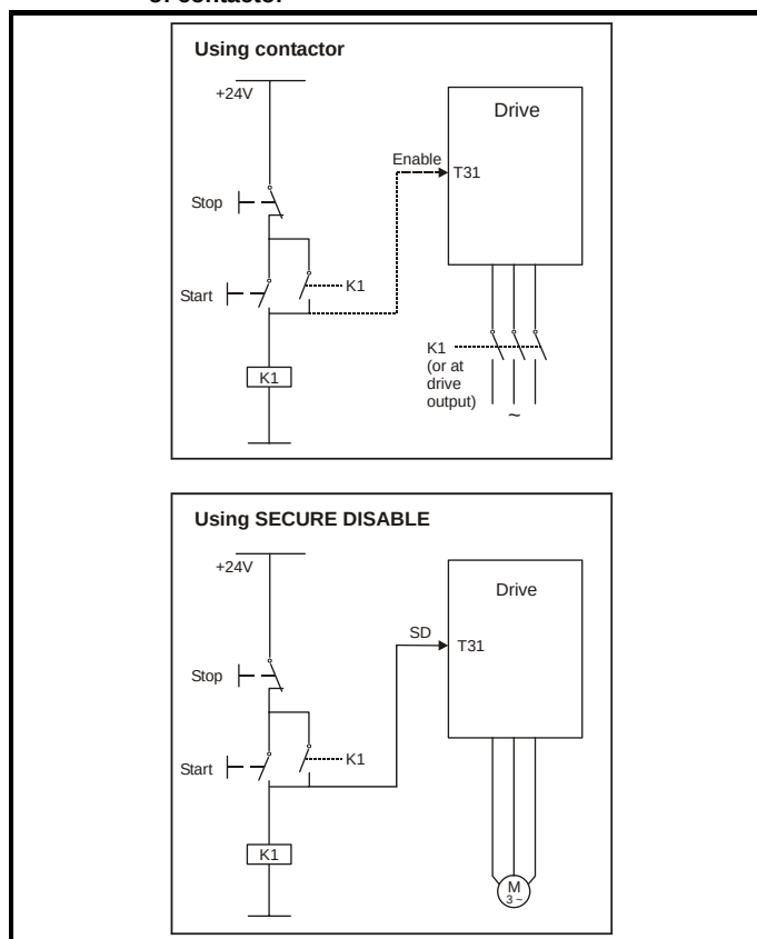
Figure 6-40 Start / stop control EN954-1 category B - replacement of contactor
