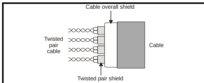
Figure 6-19 Feedback cable connections
