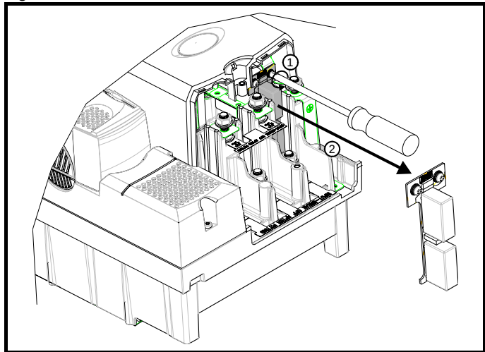
Figure 6-15 Removal of internal EMC filter
