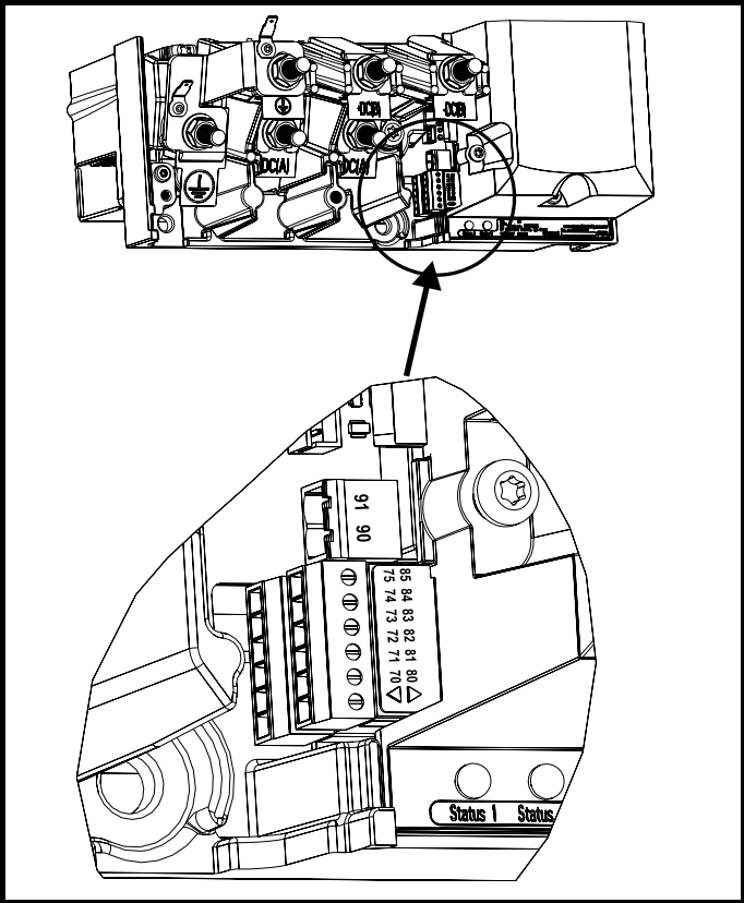
Figure 6-31 Location of SPMC (rectifier) control terminals
