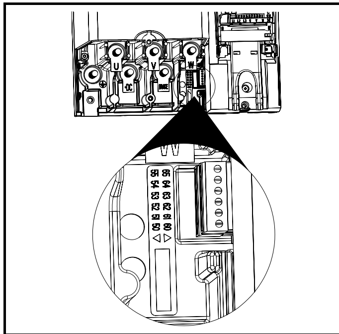
Figure 6-38 SPMA low voltage DC mode enable connections
