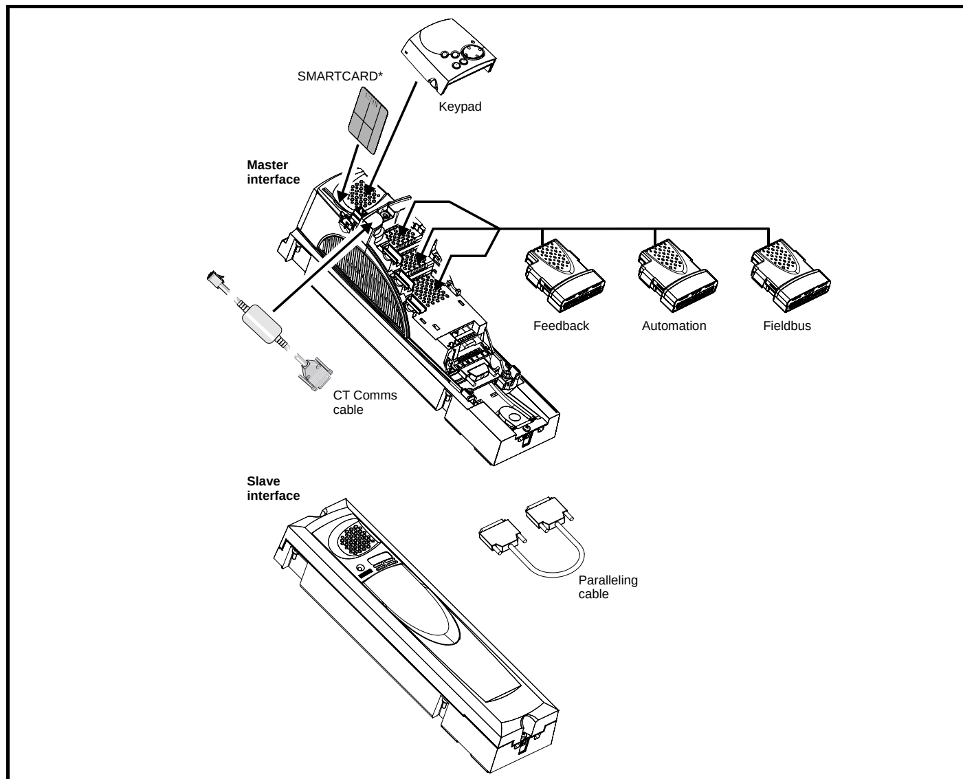
Figure 3-3 Control options available with Unidrive SPM
