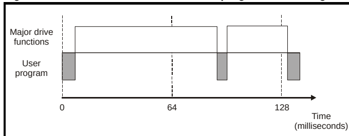
Figure 12-1 Unidrive SPM Onboard PLC program scheduling
