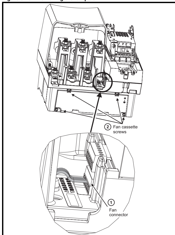
Figure 5-26 Removing the fan part 2
