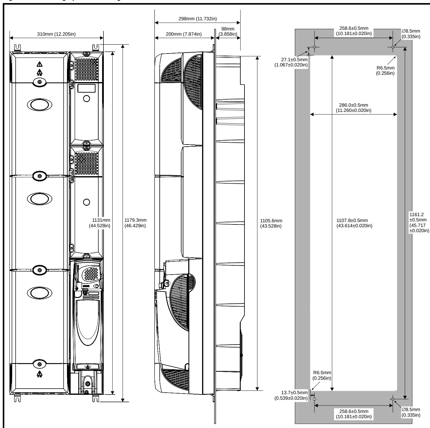
Figure 5-11 Through-panel mounting the Unidrive SPMA
