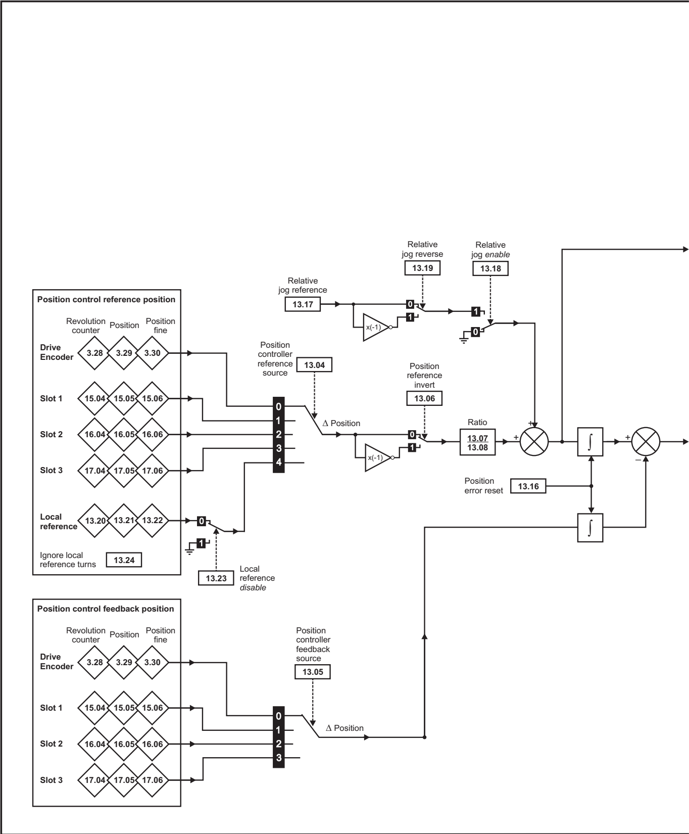
Figure 13-20 Menu 13 Open-loop logic diagram
