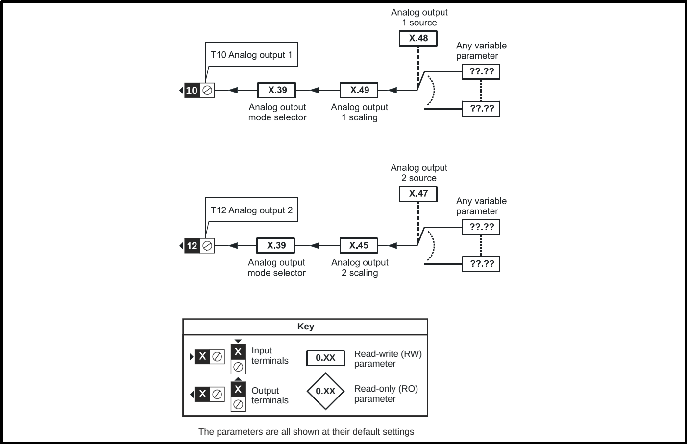
Figure 13-37 SM-PELV analog output logic diagram
