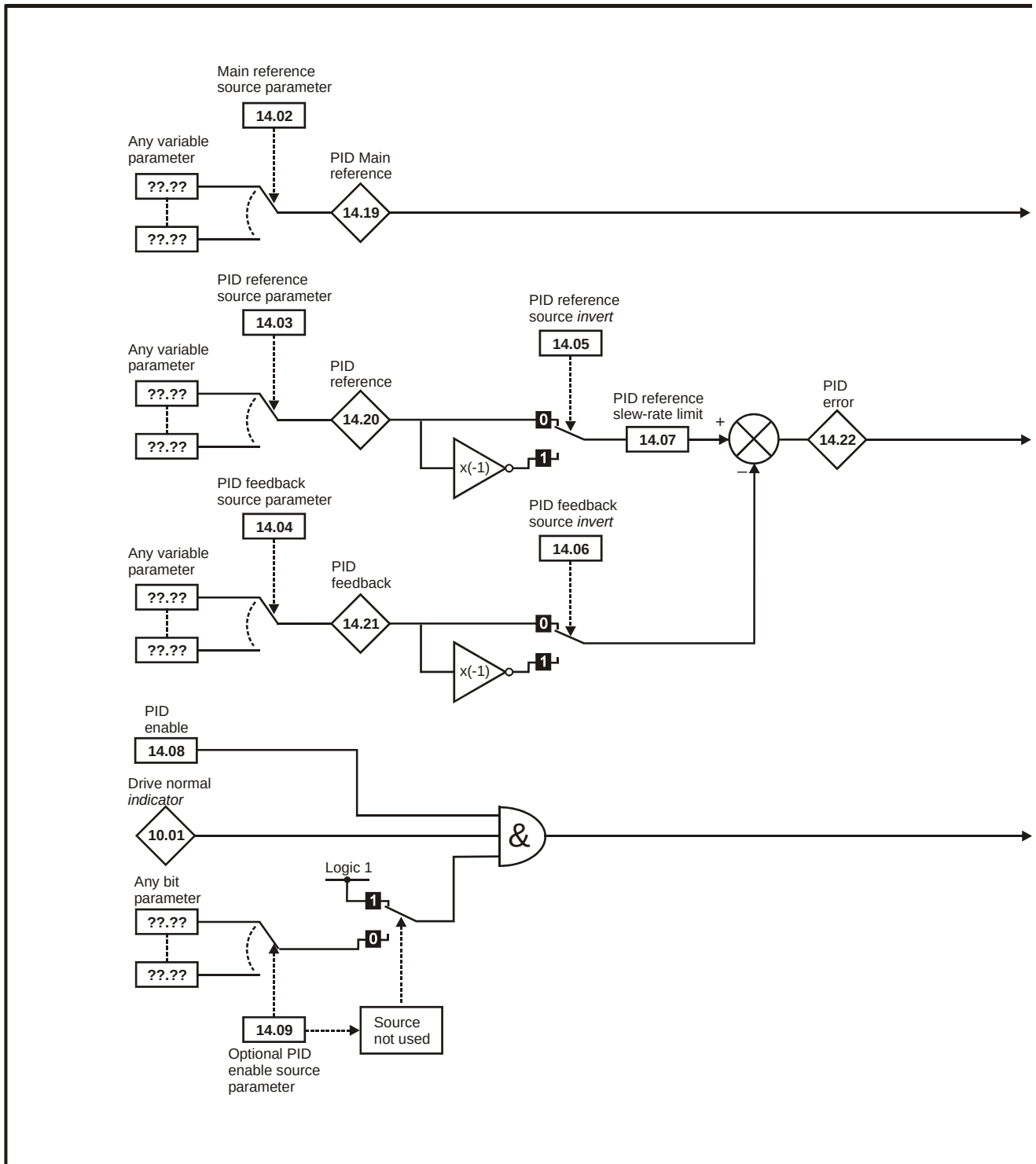
Figure 13-22 Menu 14 Logic diagram
