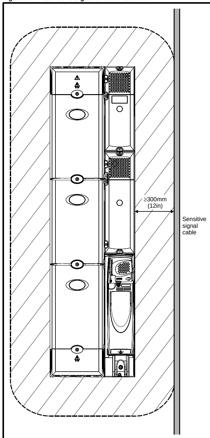
Figure 6-21 Sensitive signal circuit clearance
