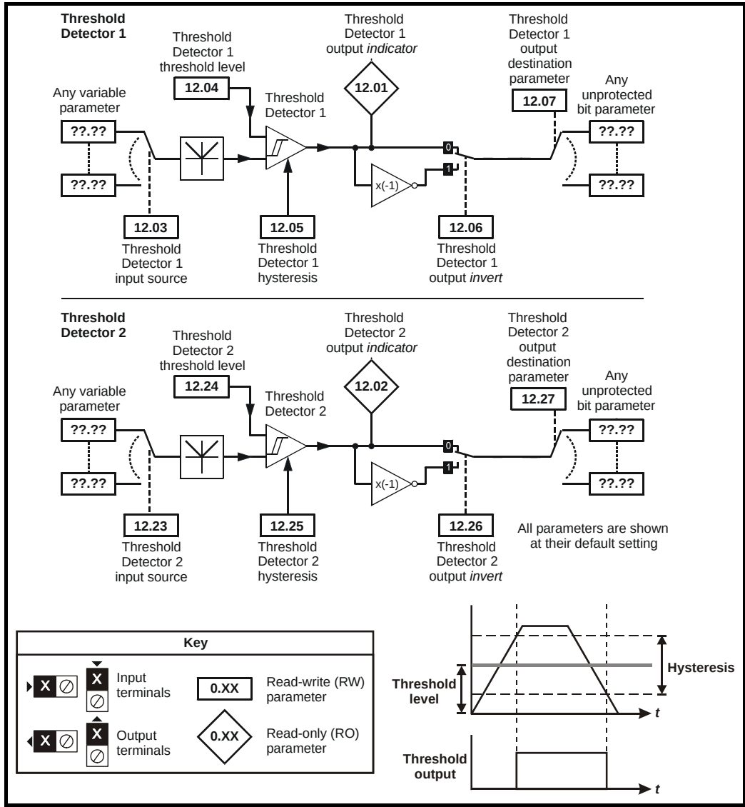
Figure 13-14 Menu 12 logic diagram
