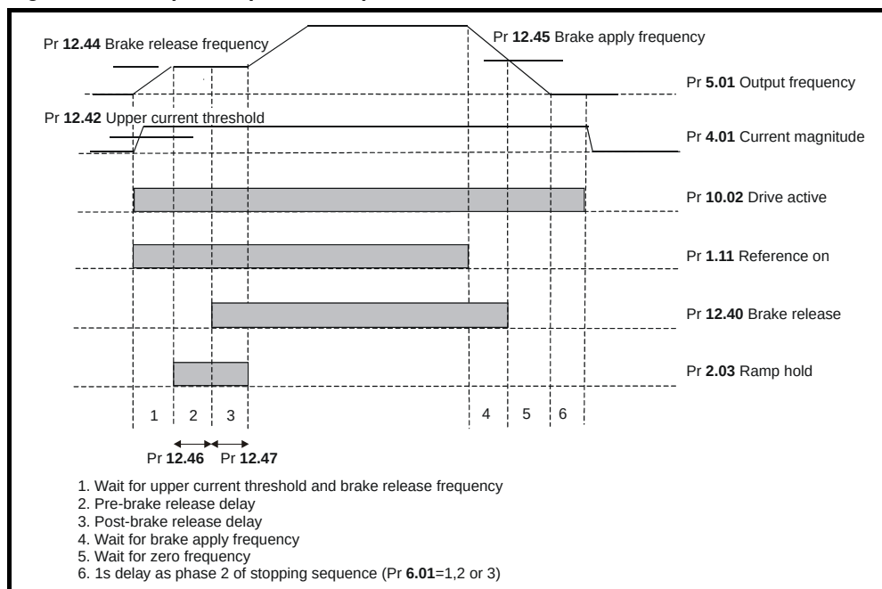
Figure 13-17 Open-loop brake sequence
