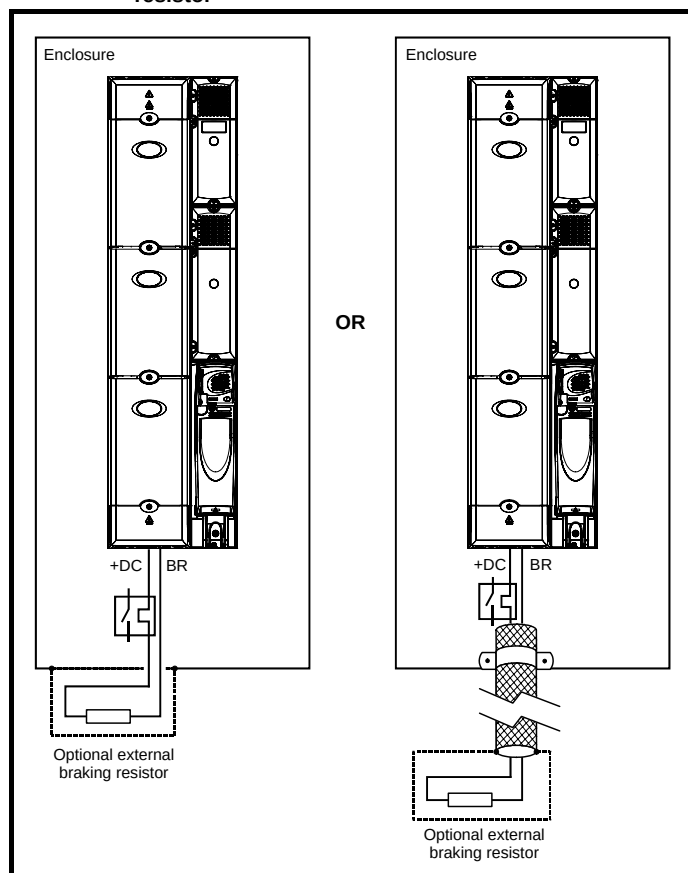
Figure 6-24 Shielding requirements of optional external braking resistor
