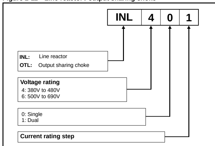
Figure 2-11 Line reactor / output sharing choke
