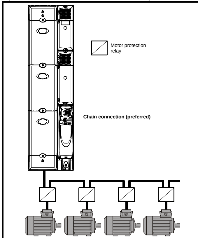
Figure 6-11 Preferred chain connection for multiple motors
