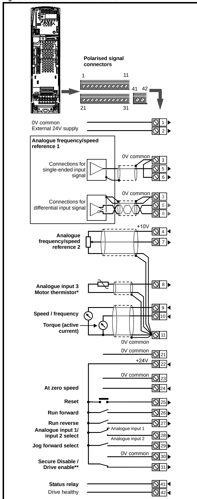
Figure 6-35 Default terminal functions
