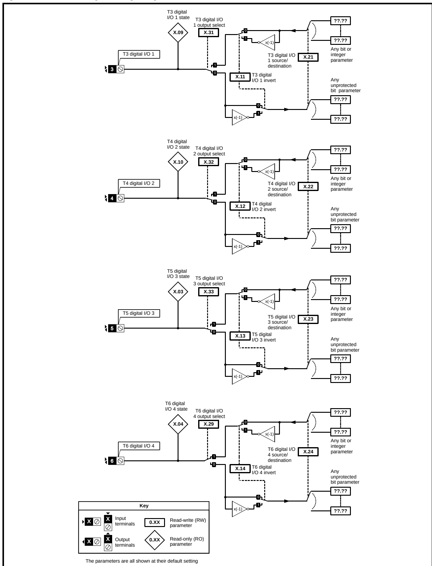
Figure 13-33 SM-PELV digital I/O logic diagram
