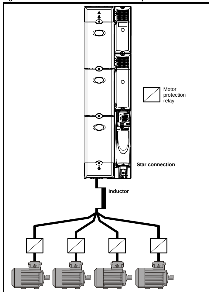
Figure 6-12 Alternative connection for multiple motors
