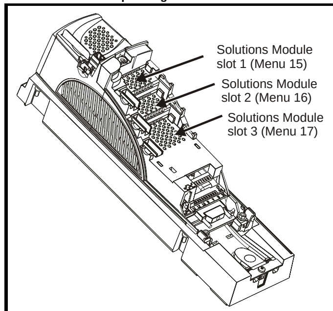
Figure 13-23 Location of Solutions Module slots and their corresponding menu numbers
