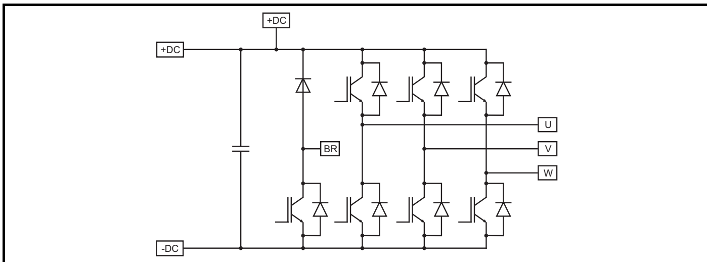
Figure 2-6 SPMA inverter schematic
