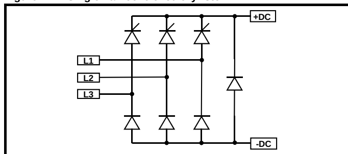
Figure 2-1 Single half controlled thyristor
