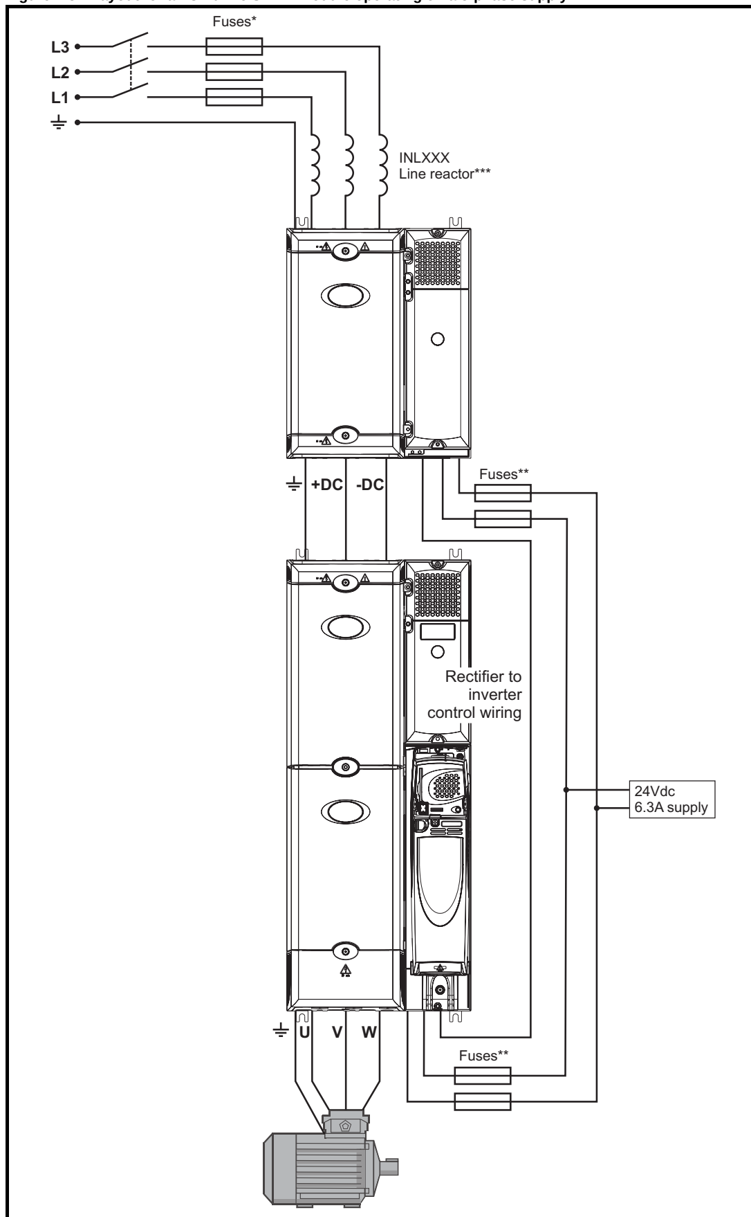
Figure 4-3 Layout for an Unidrive SPMD module operating on a 3-phase supply
