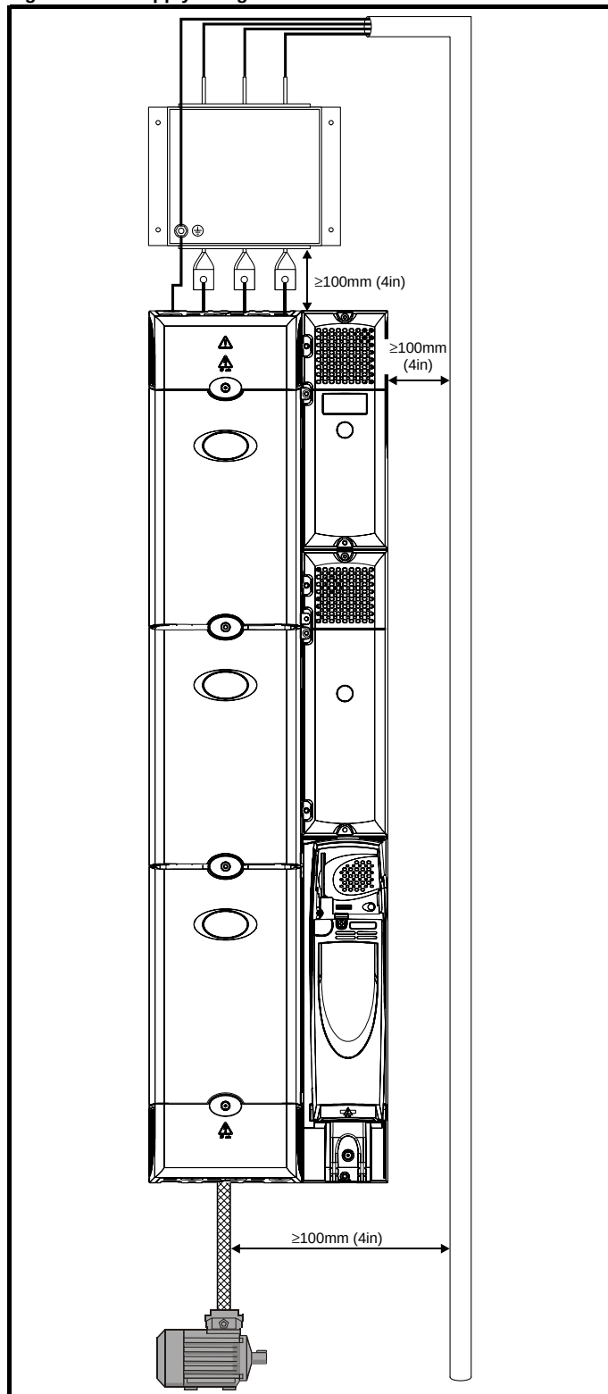
Figure 6-20 Supply and ground cable clearance
