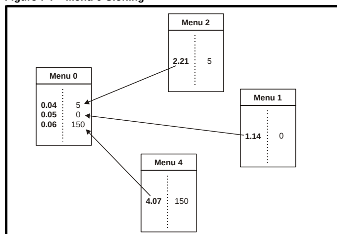
Figure 7-7 Menu 0 Cloning
