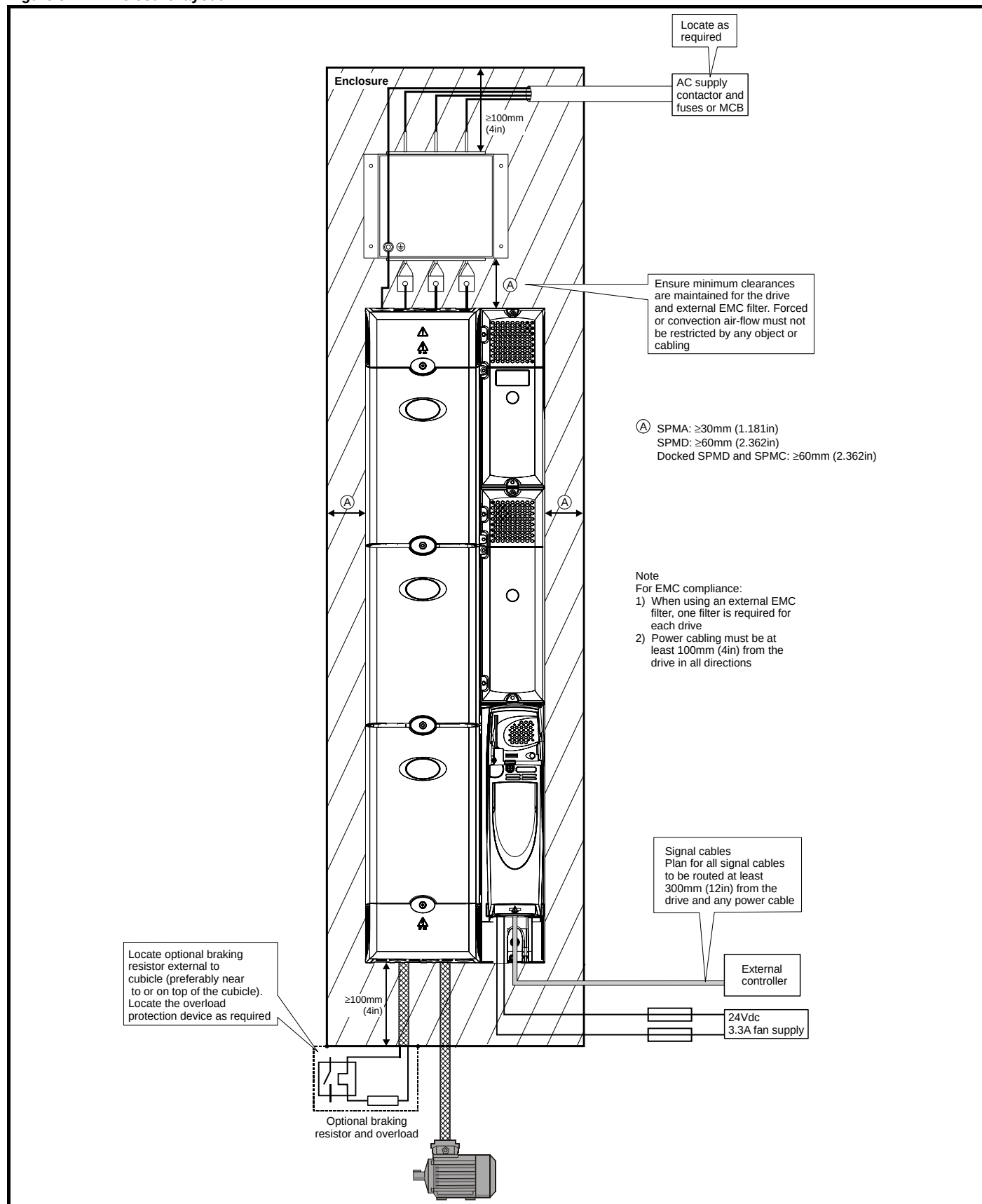
Figure 5-22 Enclosure layout
