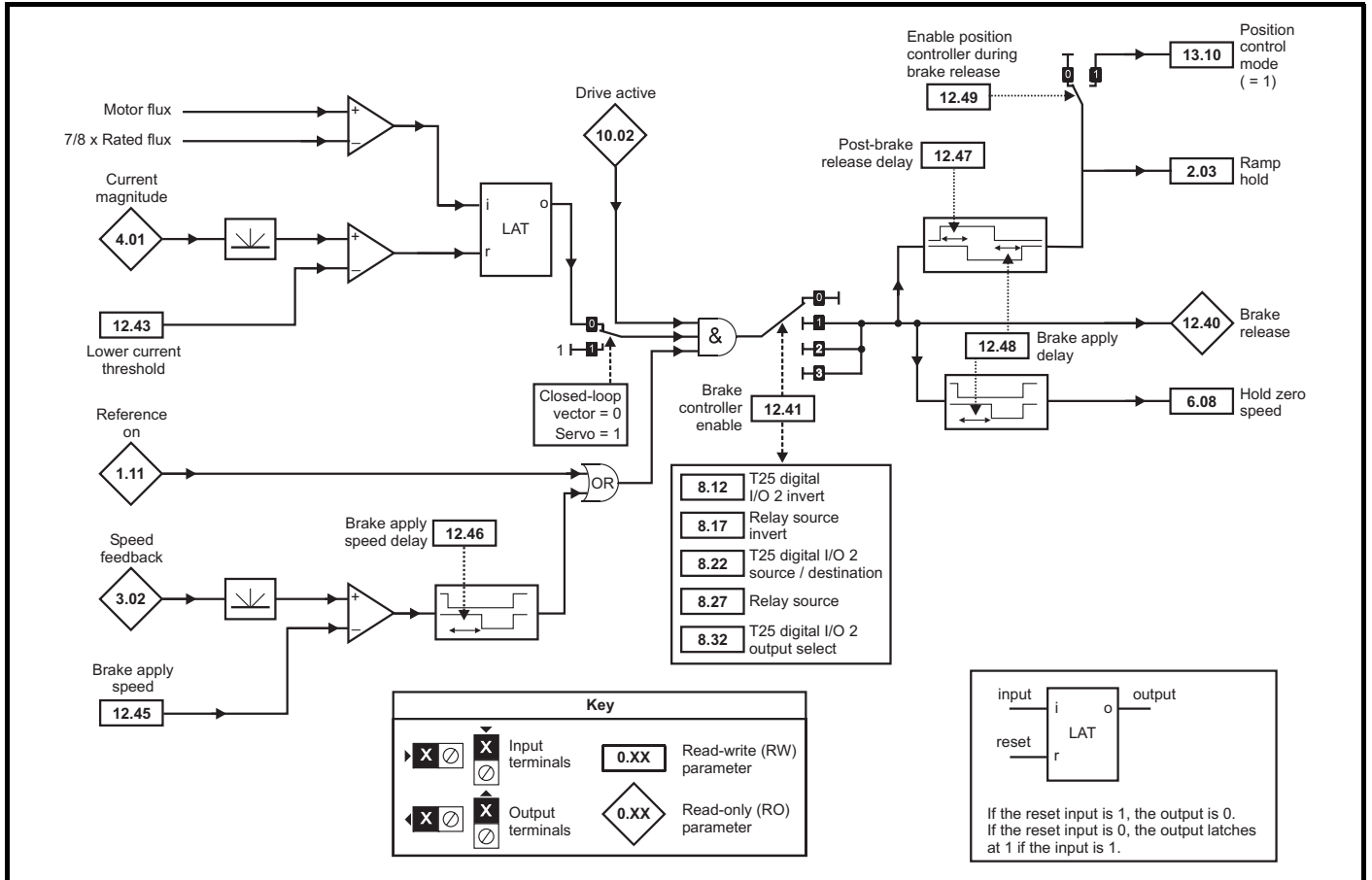
Figure 13-19 Closed-loop brake sequence
