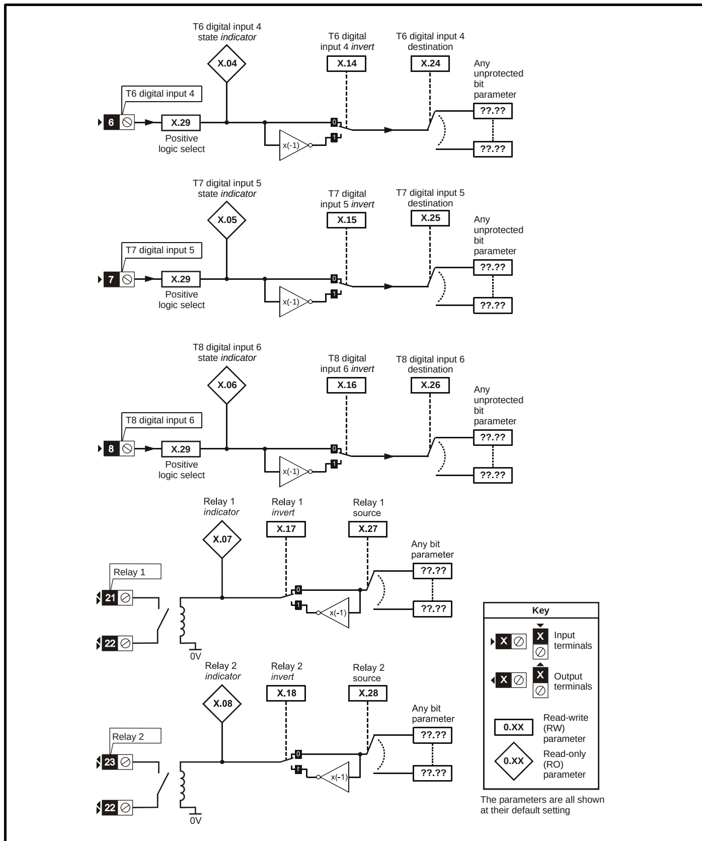
Figure 13-29 SM-I/O Plus digital logic diagram 2
