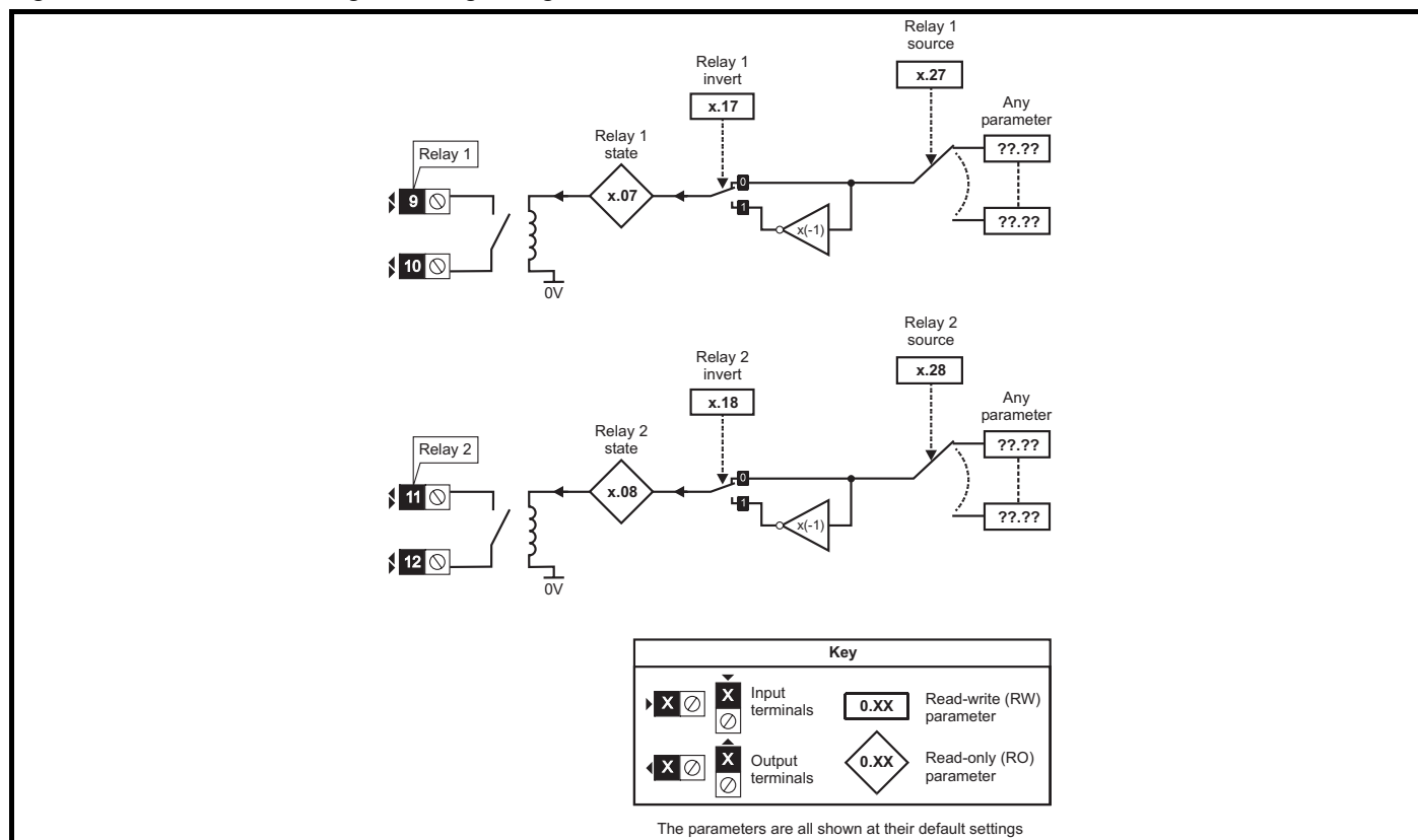
Figure 13-39 SM-I/O 120V digital I/O logic diagram
