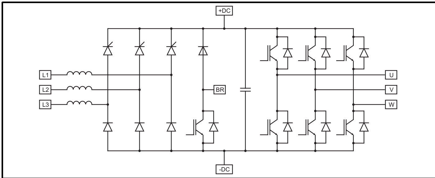
Figure 2-5 SPMA inverter schematic
