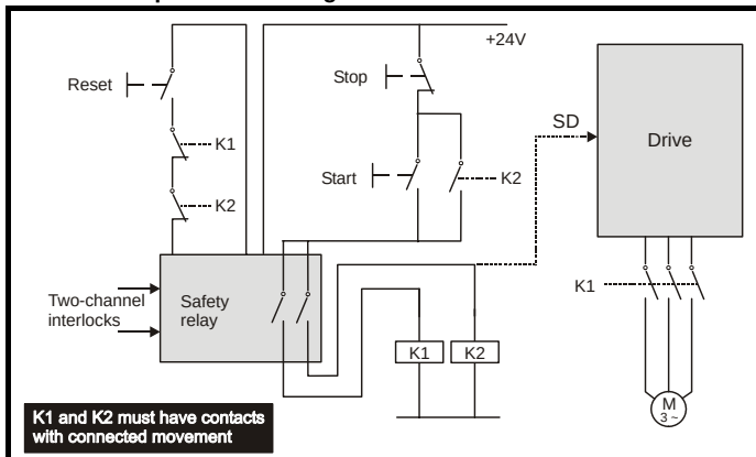
Figure 6-43 Use of contactor and relay to avoid the need for protected wiring
