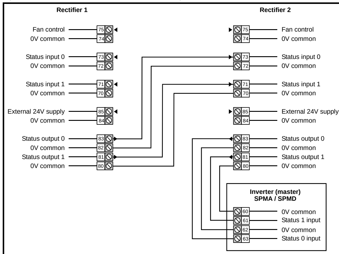
Figure 6-33 Parallel rectifier control terminals and descriptions
