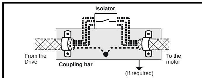
Figure 6-28 Connecting the motor cable to an isolator switch
