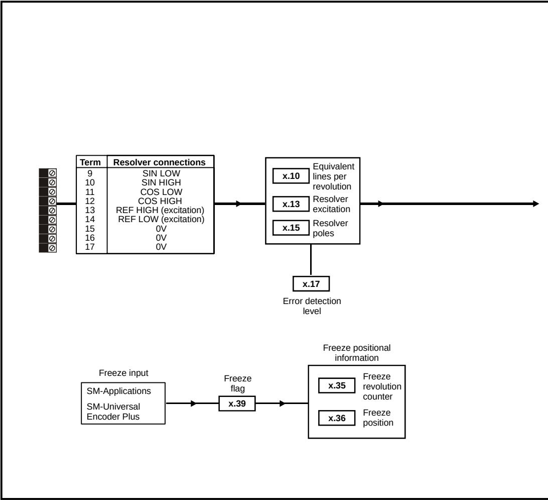
Figure 13-25 SM-Resolver logic diagram
