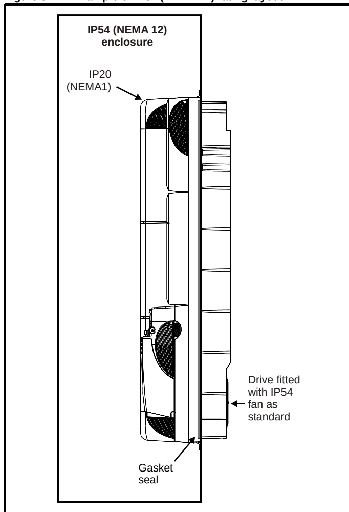
Figure 5-27 Example of IP54 (NEMA 12) rating layout
