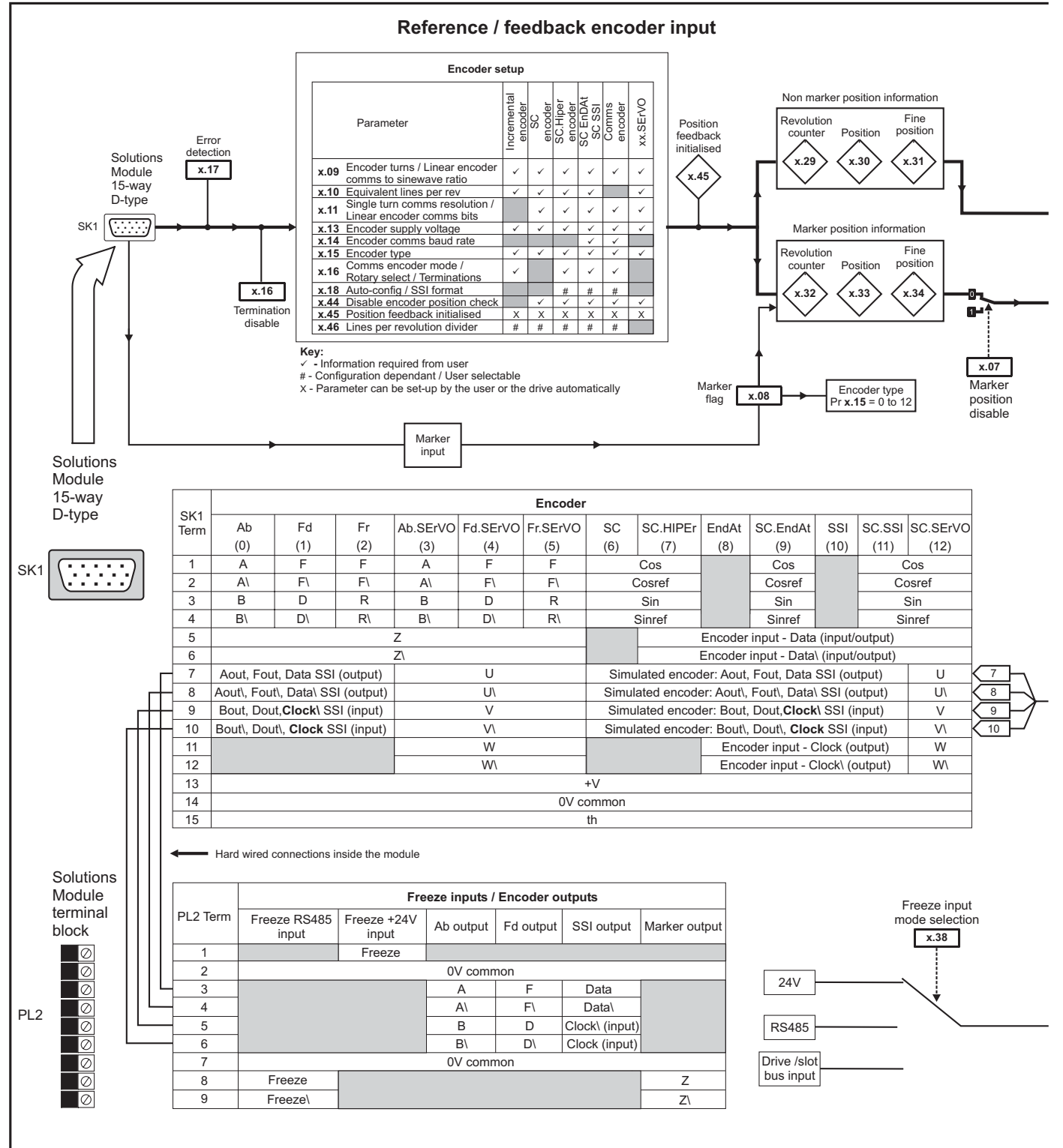
Figure 13-24 SM-Universal Encoder Plus logic diagram
