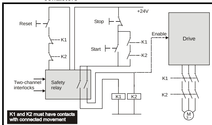
Figure 6-41 Category 3 interlock using electromechanical safety contactors
