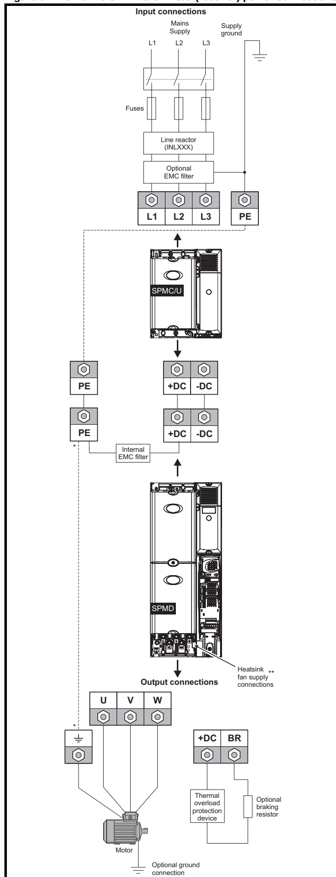
Figure 6-2 Unidrive SPMD & SPMC/U (rectifier) power connections
