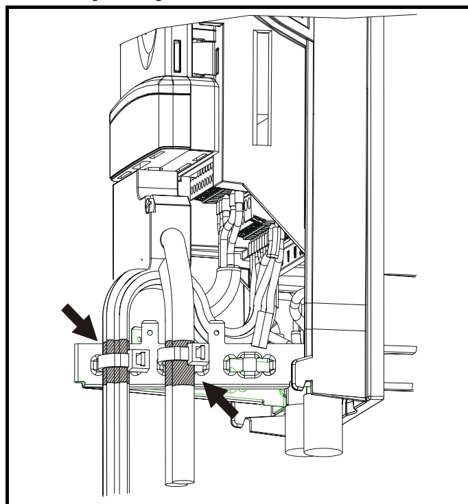
Figure 6-26 Grounding of SPMC/U signal cables
