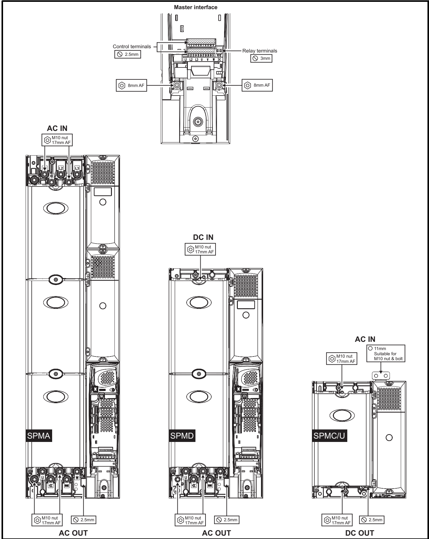
Figure 5-30 Locations of the power and ground terminals on Unidrive SPM
