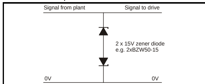
Figure 6-30 Surge suppression for analogue and bipolar inputs and outputs
