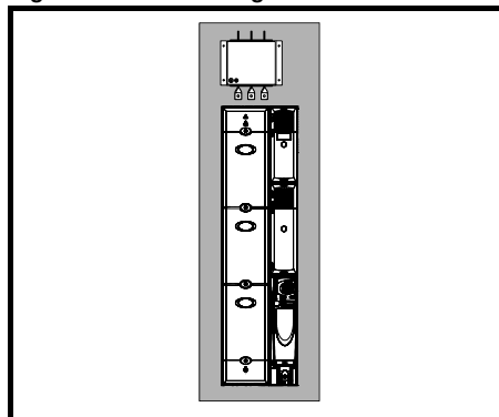
Figure 5-28 Mounting the external EMC filter
