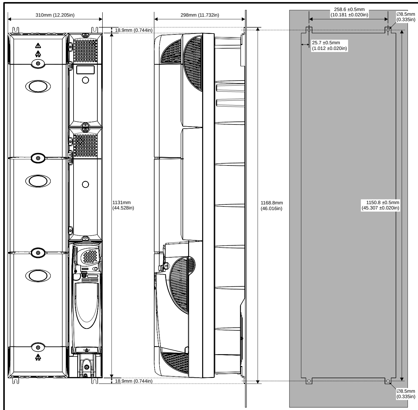
Figure 5-7 Surface mounting the Unidrive SPMA
