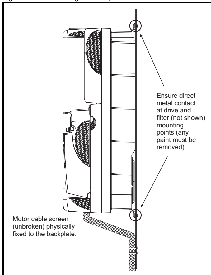
Figure 6-22 Grounding the drive, motor cable shield and filter
