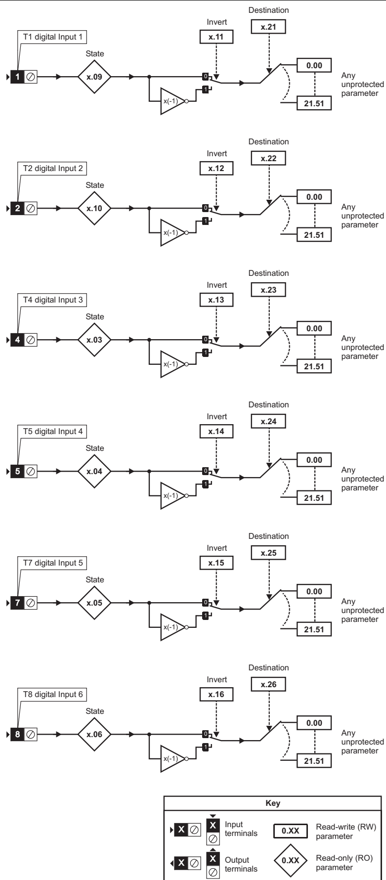
Figure 13-38 SM-I/O 120V digital input logic diagram
