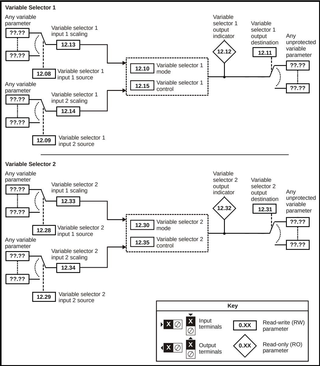
Figure 13-15 Menu 12 logic diagram (continued)
