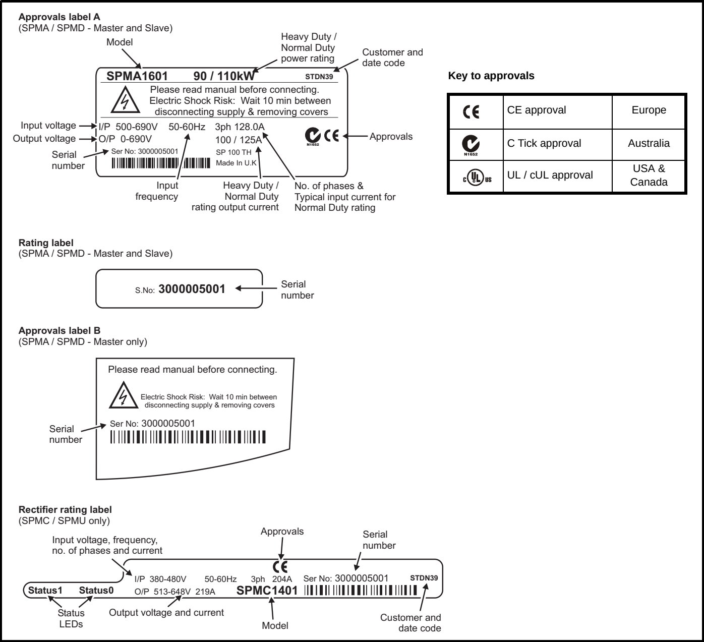
Figure 3-2 Typical drive rating labels
