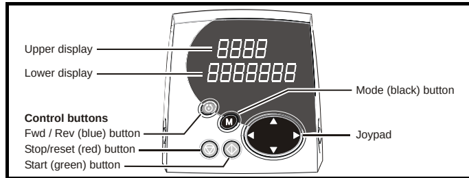
Figure 7-1 SM-Keypad
