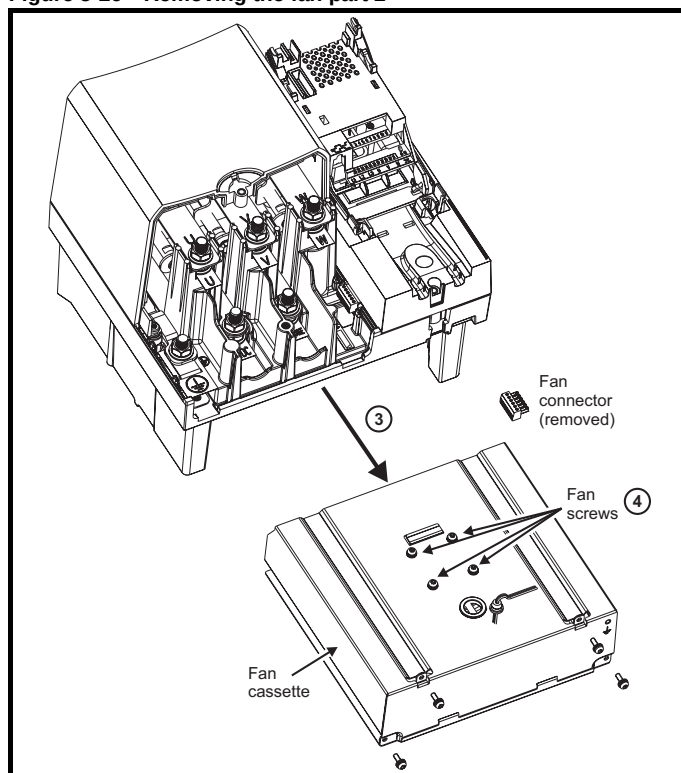
Figure 5-26 Removing the fan part 2
