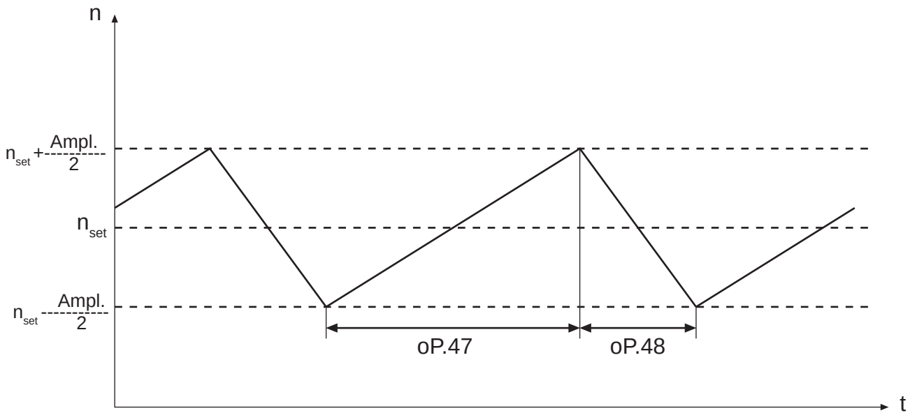
7.15.6.b Operating principle of the wobble function
