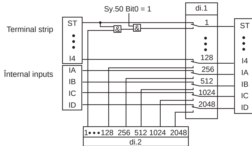
Fig. 7.3.3 Digital inputs controlled by software (di.01/di.02)
