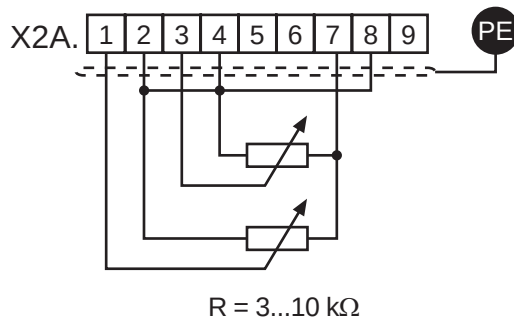
Picture 7.2.2.b Control with potentiometer and internal reference voltage
