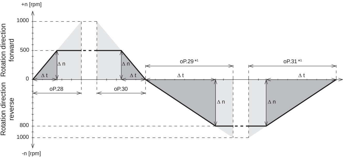
Fig. 7.4.7.2.1 Acceleration and deceleration times
