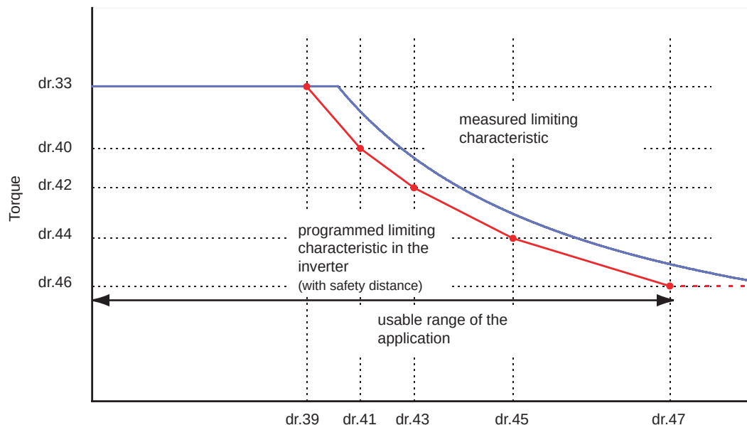
Fig. 7.8.3.2.2 Limiting characteristic
