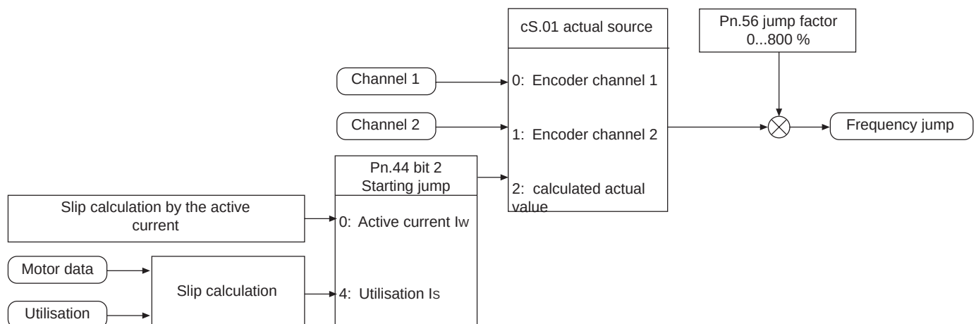
Figure 7.13.10.b Initial jump for generator operation in 1. cycle
