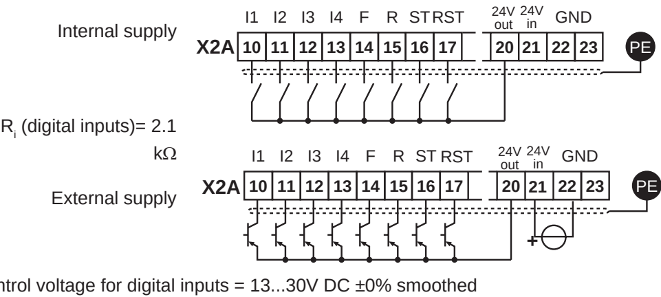
Fig. 7.3.2.a Digital inputs with PNP control (di.00 = 0)
