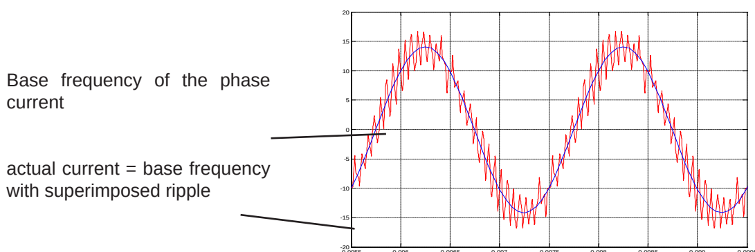
Picture 7.10.3.1 Carrier frequencies
