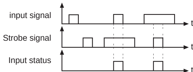
Fig. 6.3.8.c Static strobe mode 2 (di.07 = 2)
