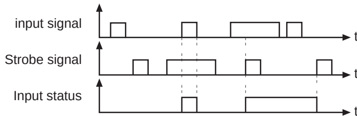
Fig. 7.3.8.b Static strobe mode 1 (di.07 = 1)
