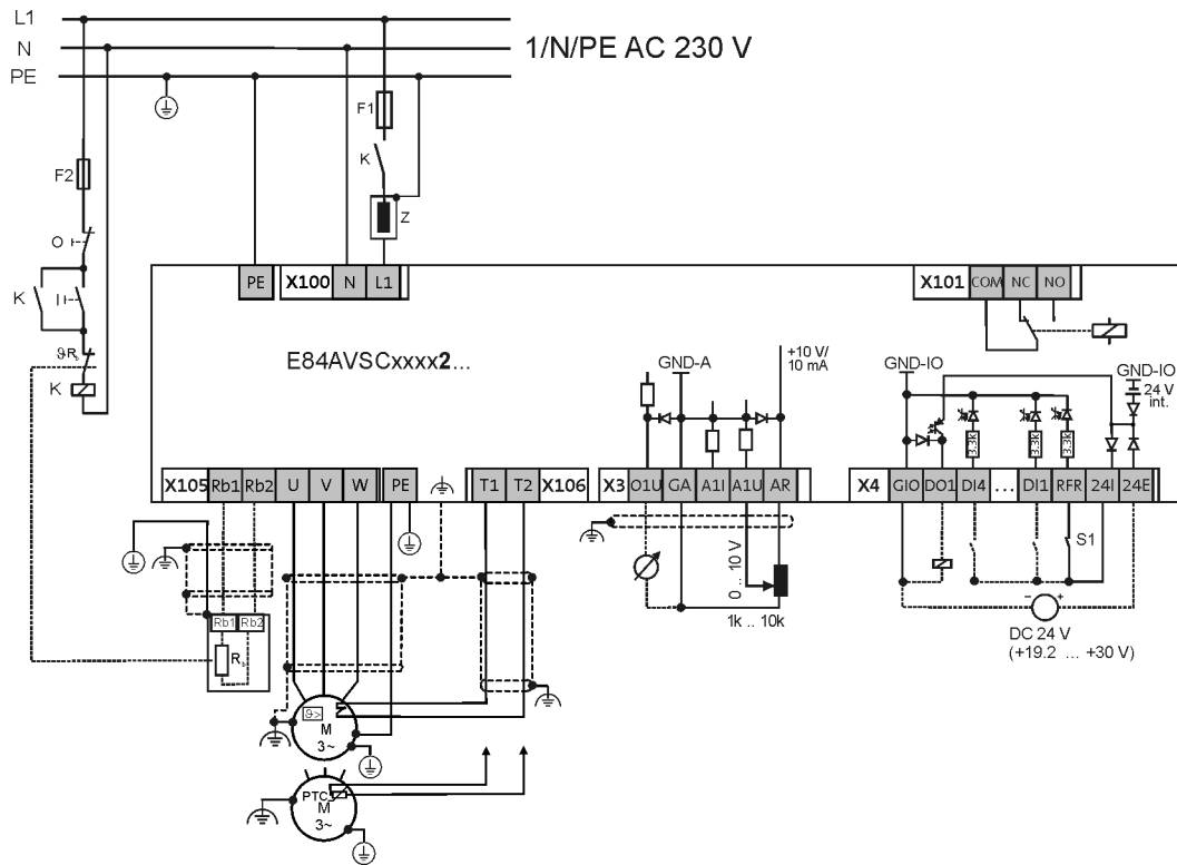
Wiring example for connecting Inverter Drives 8400 StateLine to 1 x 230V
